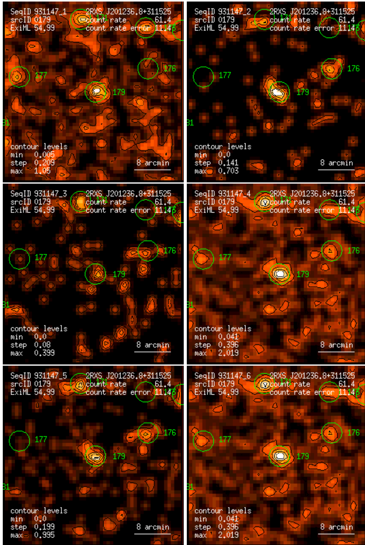
Figure 179: RASS 931147: detection 0179: band rate images, Gaussian filter: (1) PSPC channels 11 – 41, (2) 52 – 90, (3) 91 – 201, (4) 11 – 235, (5) 52 – 201, (6) 11 – 201. Broad band rates in counts/ks. Band rate contour levels in counts/ks/arcmin 2 .
