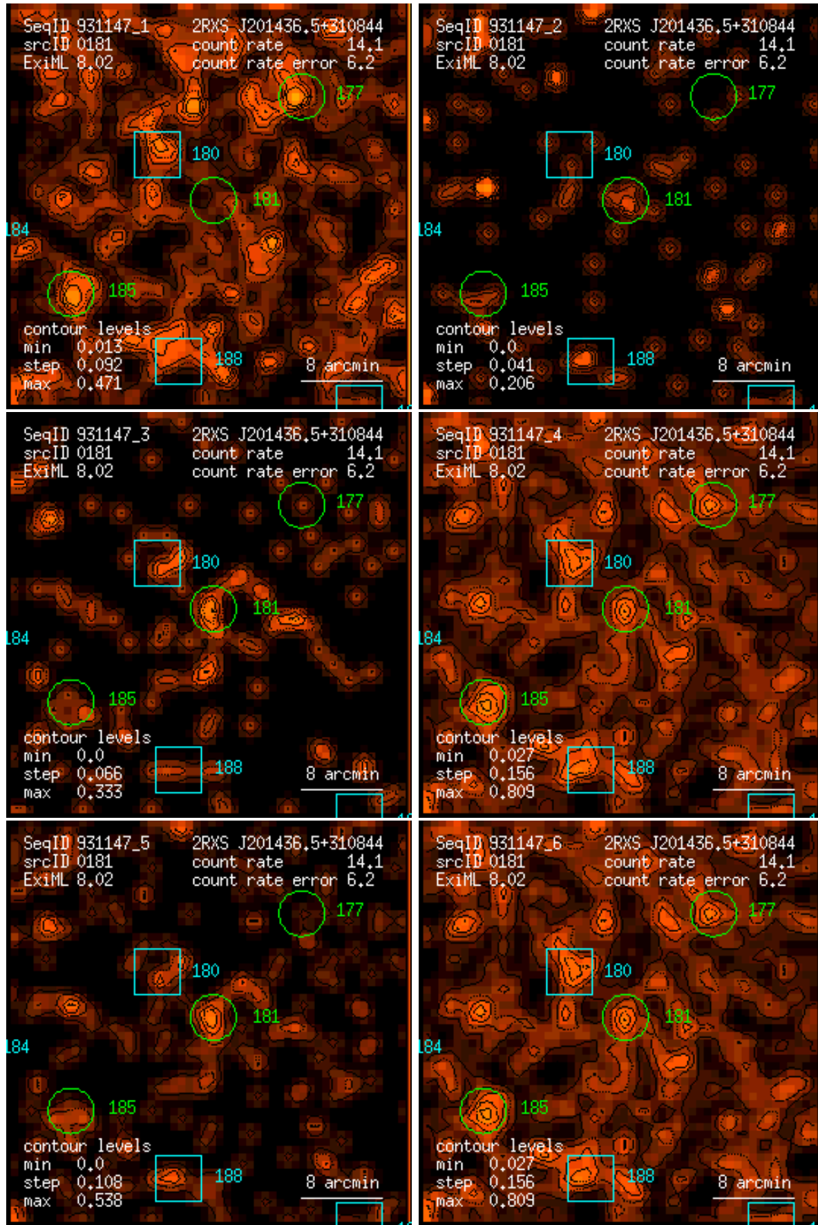
Figure 181: RASS 931147: detection 0181: band rate images, Gaussian filter: (1) PSPC channels 11 – 41, (2) 52 – 90, (3) 91 – 201, (4) 11 – 235, (5) 52 – 201, (6) 11 – 201. Broad band rates in counts/ks. Band rate contour levels in counts/ks/arcmin 2 .
