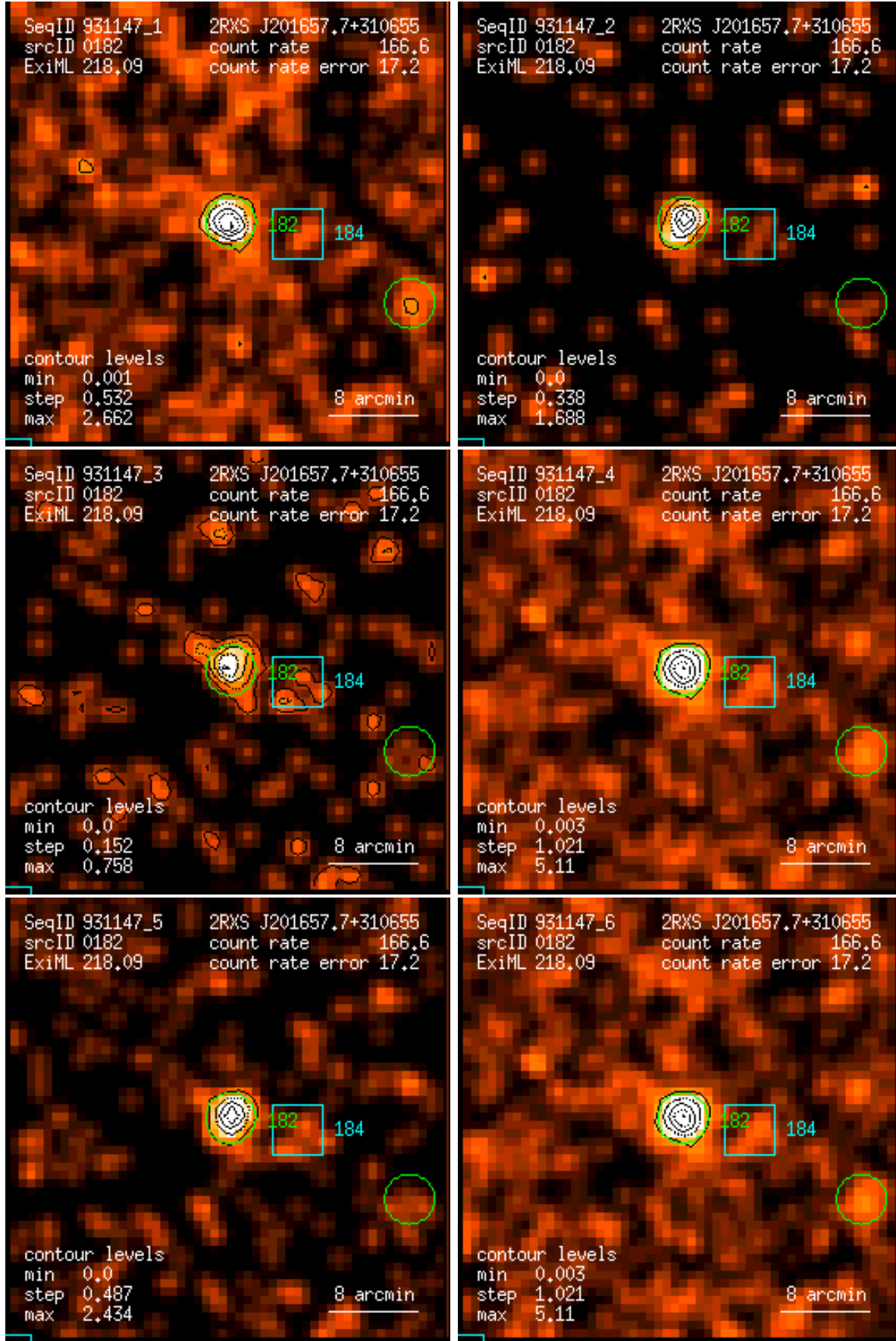
Figure 182: RASS 931147: detection 0182: band rate images, Gaussian filter: (1) PSPC channels 11 – 41, (2) 52 – 90, (3) 91 – 201, (4) 11 – 235, (5) 52 – 201, (6) 11 – 201. Broad band rates in counts/ks. Band rate contour levels in counts/ks/arcmin 2 .
