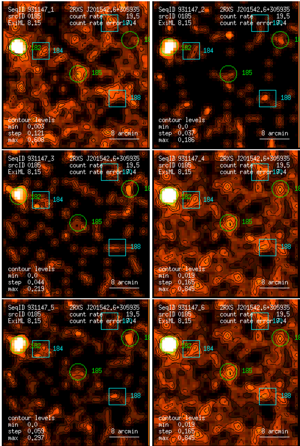
Figure 185: RASS 931147: detection 0185: band rate images, Gaussian filter: (1) PSPC channels 11 – 41, (2) 52 – 90, (3) 91 – 201, (4) 11 – 235, (5) 52 – 201, (6) 11 – 201. Broad band rates in counts/ks. Band rate contour levels in counts/ks/arcmin 2 .
