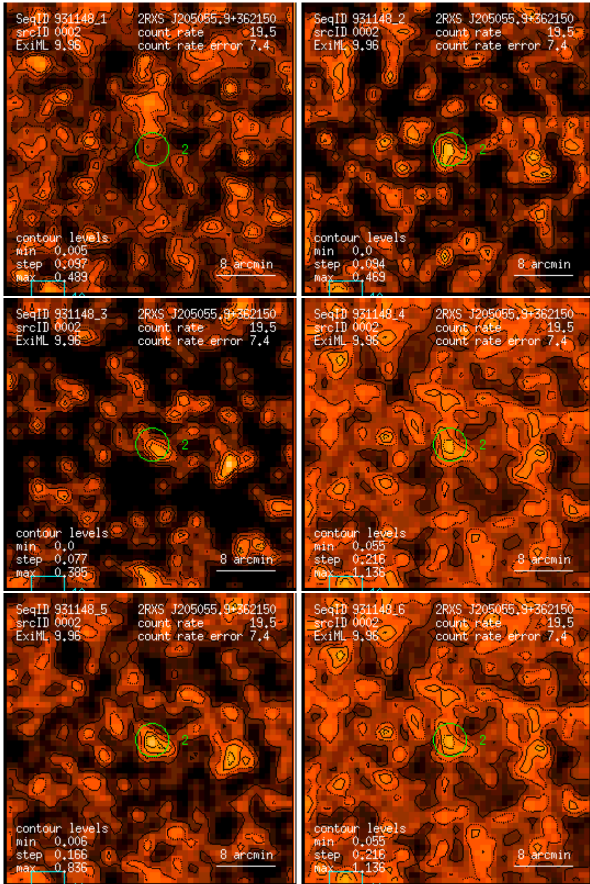
Figure 2: RASS 931148: detection 0002: band rate images, Gaussian filter: (1) PSPC channels 11 – 41, (2) 52 – 90, (3) 91 – 201, (4) 11 – 235, (5) 52 – 201, (6) 11 – 201. Broad band rates in counts/ks. Band rate contour levels in counts/ks/arcmin 2 .
