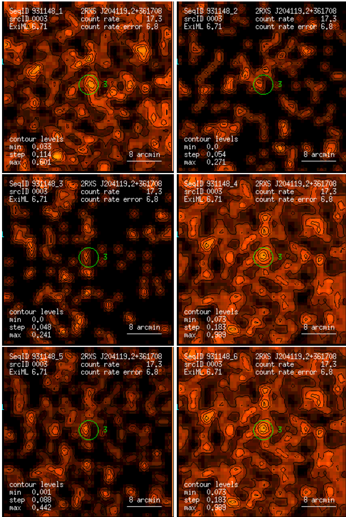
Figure 3: RASS 931148: detection 0003: band rate images, Gaussian filter: (1) PSPC channels 11 – 41, (2) 52 – 90, (3) 91 – 201, (4) 11 – 235, (5) 52 – 201, (6) 11 – 201. Broad band rates in counts/ks. Band rate contour levels in counts/ks/arcmin 2 .
