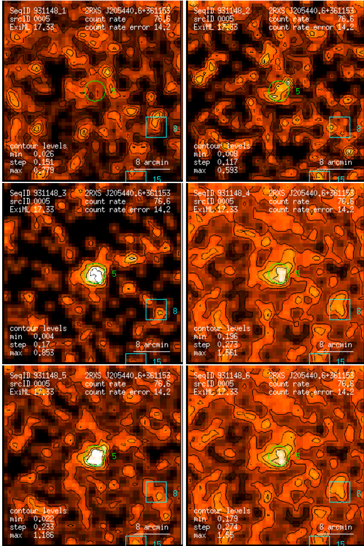
Figure 5: RASS 931148: detection 0005: band rate images, Gaussian filter: (1) PSPC channels 11 – 41, (2) 52 – 90, (3) 91 – 201, (4) 11 – 235, (5) 52 – 201, (6) 11 – 201. Broad band rates in counts/ks. Band rate contour levels in counts/ks/arcmin 2 .
