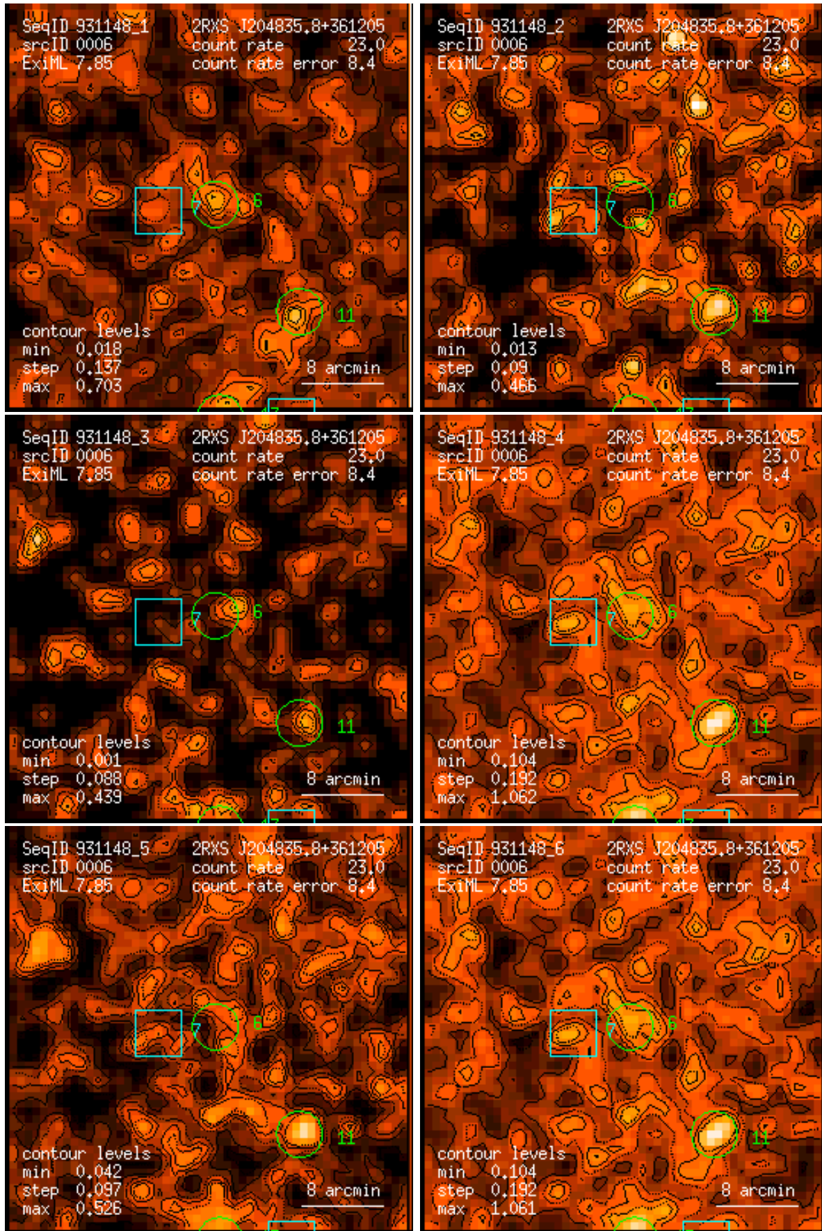
Figure 6: RASS 931148: detection 0006: band rate images, Gaussian filter: (1) PSPC channels 11 – 41, (2) 52 – 90, (3) 91 – 201, (4) 11 – 235, (5) 52 – 201, (6) 11 – 201. Broad band rates in counts/ks. Band rate contour levels in counts/ks/arcmin 2 .
