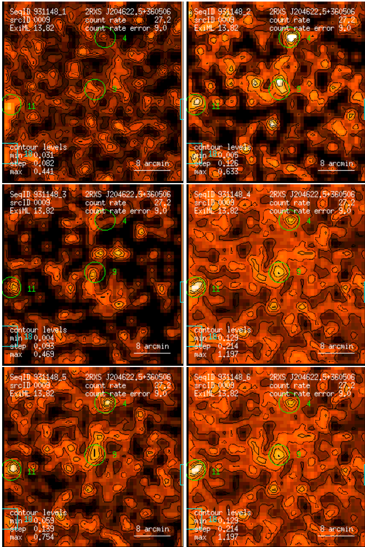
Figure 9: RASS 931148: detection 0009: band rate images, Gaussian filter: (1) PSPC channels 11 – 41, (2) 52 – 90, (3) 91 – 201, (4) 11 – 235, (5) 52 – 201, (6) 11 – 201. Broad band rates in counts/ks. Band rate contour levels in counts/ks/arcmin 2 .
