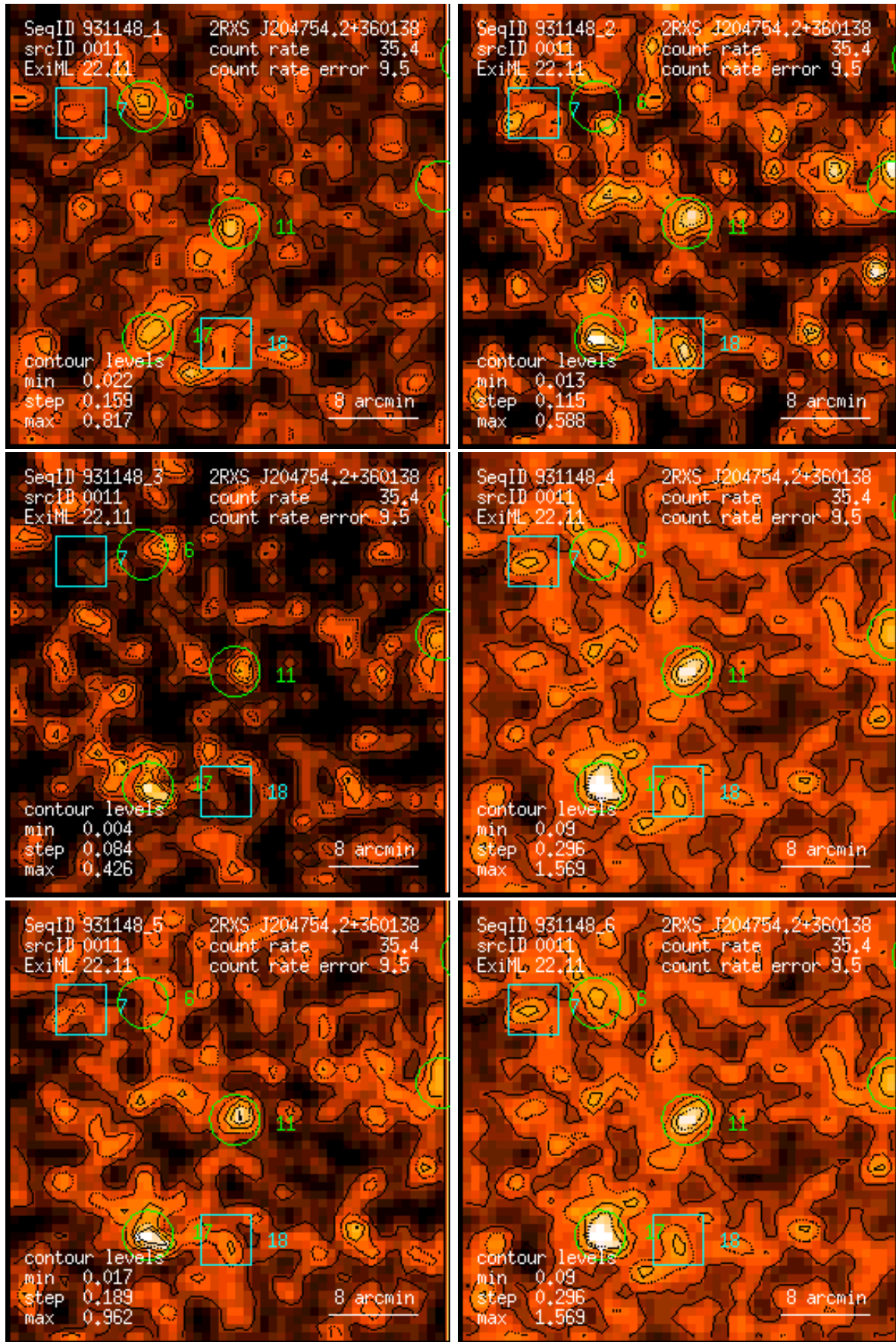
Figure 11: RASS 931148: detection 0011: band rate images, Gaussian filter: (1) PSPC channels 11 – 41, (2) 52 – 90, (3) 91 – 201, (4) 11 – 235, (5) 52 – 201, (6) 11 – 201. Broad band rates in counts/ks. Band rate contour levels in counts/ks/arcmin 2 .
