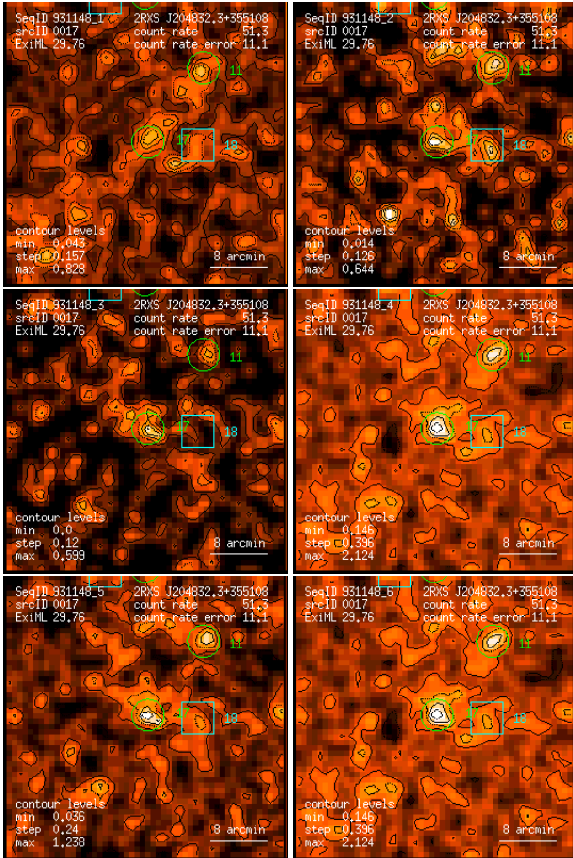
Figure 17: RASS 931148: detection 0017: band rate images, Gaussian filter: (1) PSPC channels 11 – 41, (2) 52 – 90, (3) 91 – 201, (4) 11 – 235, (5) 52 – 201, (6) 11 – 201. Broad band rates in counts/ks. Band rate contour levels in counts/ks/arcmin 2 .
