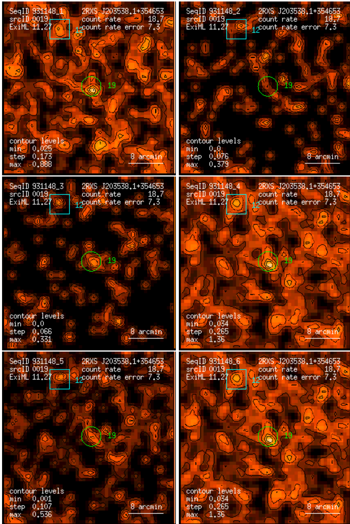
Figure 19: RASS 931148: detection 0019: band rate images, Gaussian filter: (1) PSPC channels 11 – 41, (2) 52 – 90, (3) 91 – 201, (4) 11 – 235, (5) 52 – 201, (6) 11 – 201. Broad band rates in counts/ks. Band rate contour levels in counts/ks/arcmin 2 .
