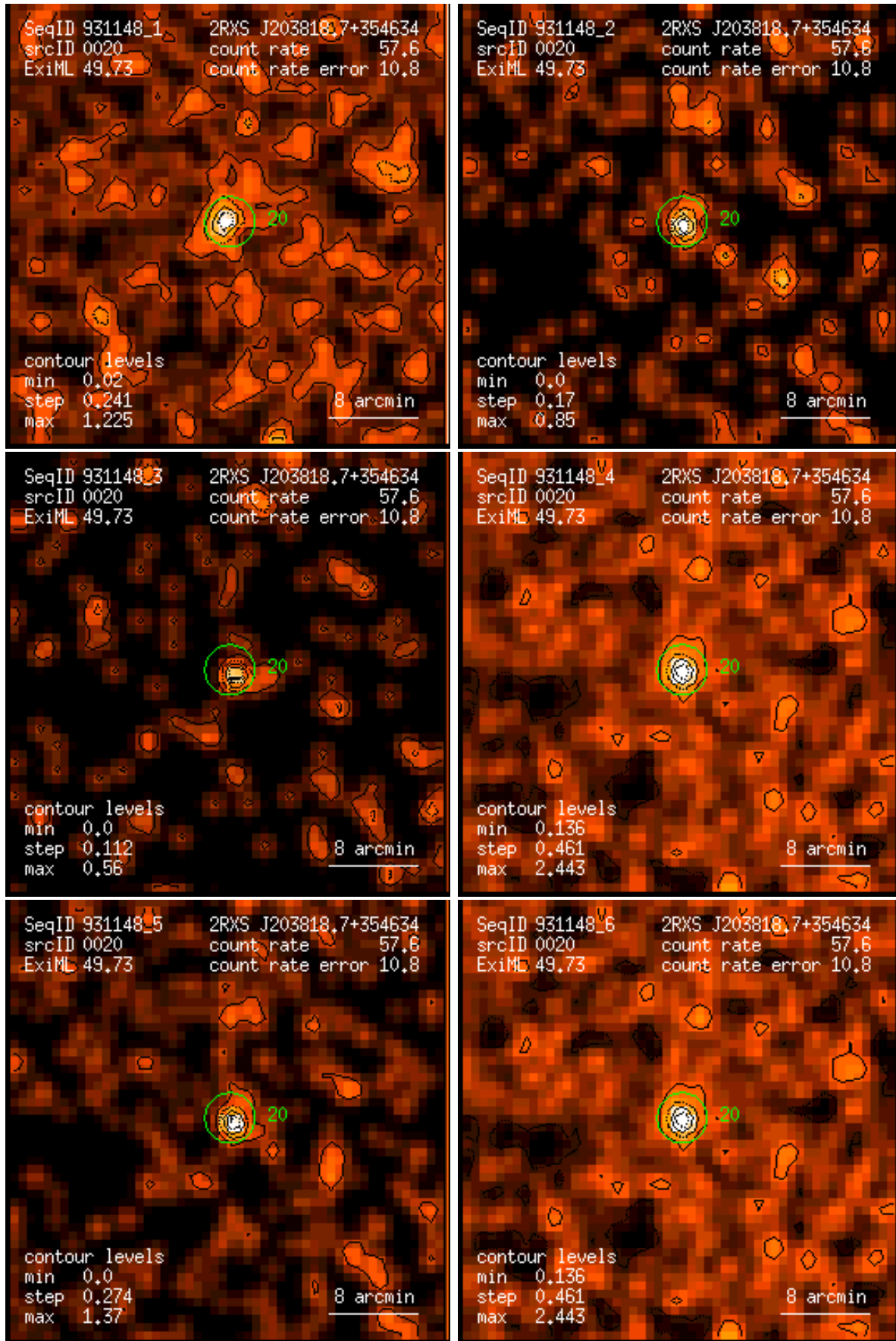
Figure 20: RASS 931148: detection 0020: band rate images, Gaussian filter: (1) PSPC channels 11 – 41, (2) 52 – 90, (3) 91 – 201, (4) 11 – 235, (5) 52 – 201, (6) 11 – 201. Broad band rates in counts/ks. Band rate contour levels in counts/ks/arcmin 2 .
