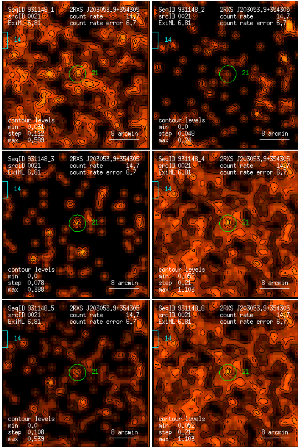
Figure 21: RASS 931148: detection 0021: band rate images, Gaussian filter: (1) PSPC channels 11 – 41, (2) 52 – 90, (3) 91 – 201, (4) 11 – 235, (5) 52 – 201, (6) 11 – 201. Broad band rates in counts/ks. Band rate contour levels in counts/ks/arcmin 2 .
