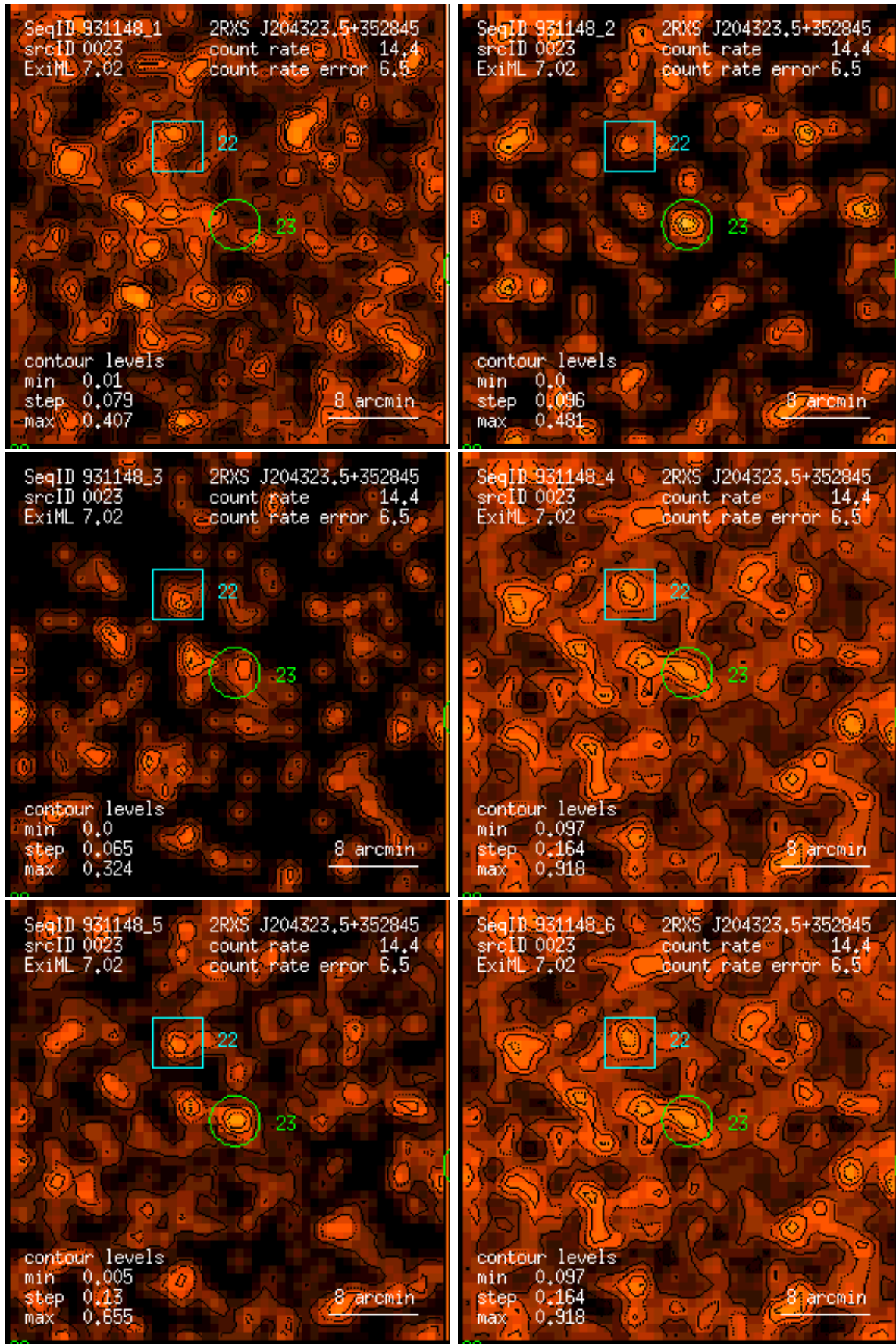
Figure 23: RASS 931148: detection 0023: band rate images, Gaussian filter: (1) PSPC channels 11 – 41, (2) 52 – 90, (3) 91 – 201, (4) 11 – 235, (5) 52 – 201, (6) 11 – 201. Broad band rates in counts/ks. Band rate contour levels in counts/ks/arcmin 2 .
