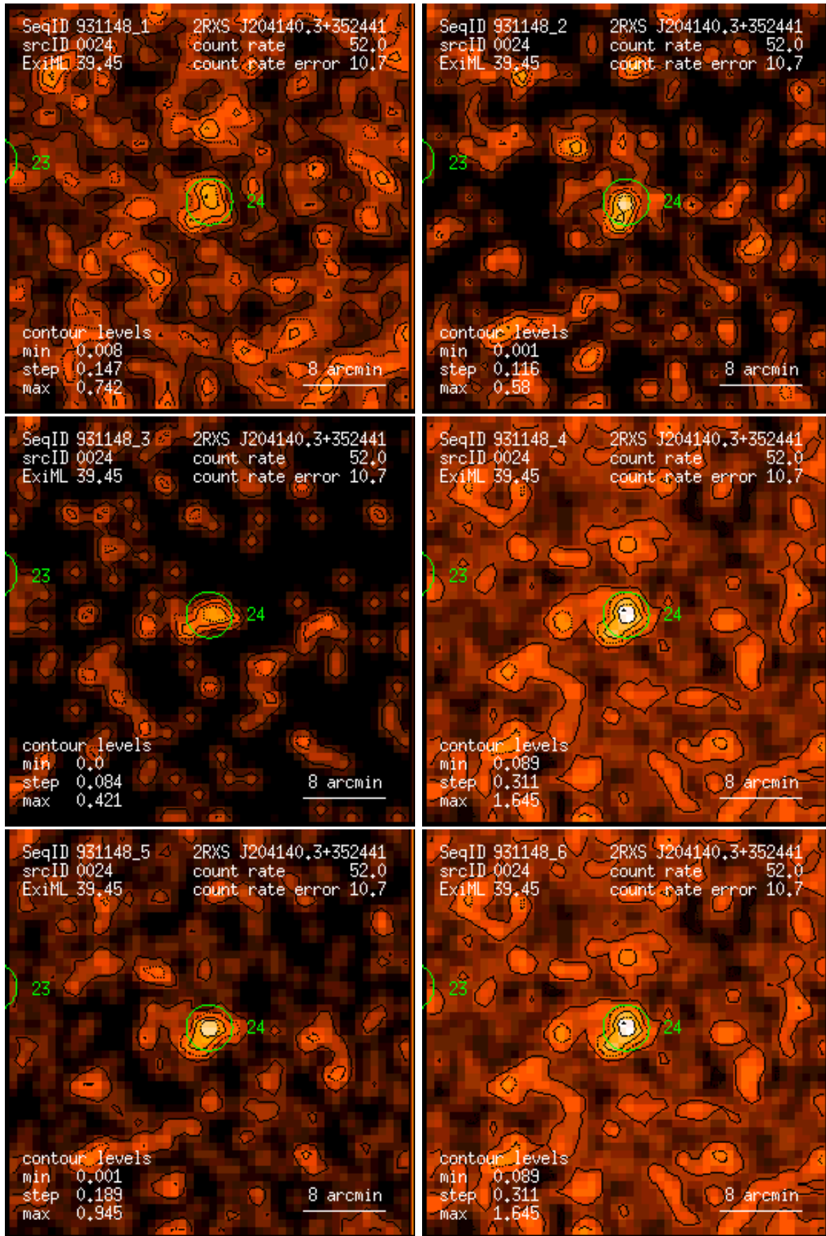
Figure 24: RASS 931148: detection 0024: band rate images, Gaussian filter: (1) PSPC channels 11 – 41, (2) 52 – 90, (3) 91 – 201, (4) 11 – 235, (5) 52 – 201, (6) 11 – 201. Broad band rates in counts/ks. Band rate contour levels in counts/ks/arcmin 2 .
