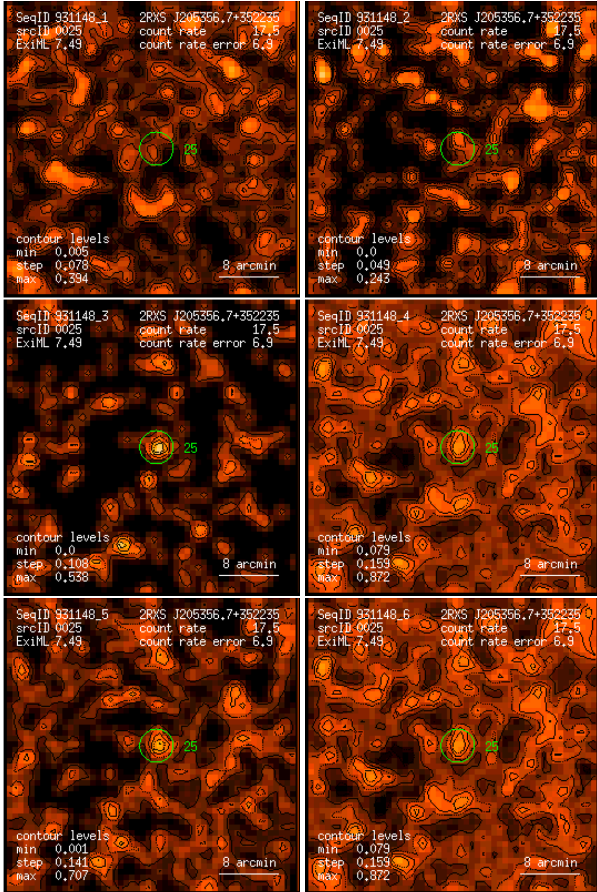
Figure 25: RASS 931148: detection 0025: band rate images, Gaussian filter: (1) PSPC channels 11 – 41, (2) 52 – 90, (3) 91 – 201, (4) 11 – 235, (5) 52 – 201, (6) 11 – 201. Broad band rates in counts/ks. Band rate contour levels in counts/ks/arcmin 2 .
