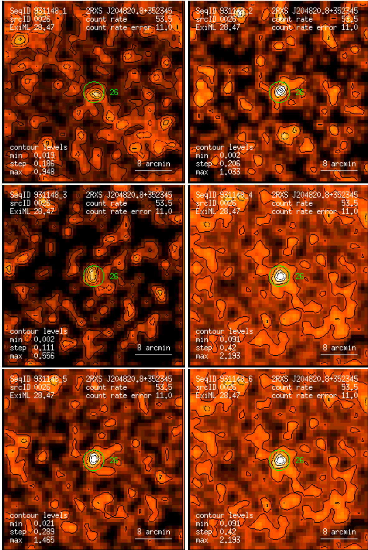
Figure 26: RASS 931148: detection 0026: band rate images, Gaussian filter: (1) PSPC channels 11 – 41, (2) 52 – 90, (3) 91 – 201, (4) 11 – 235, (5) 52 – 201, (6) 11 – 201. Broad band rates in counts/ks. Band rate contour levels in counts/ks/arcmin 2 .
