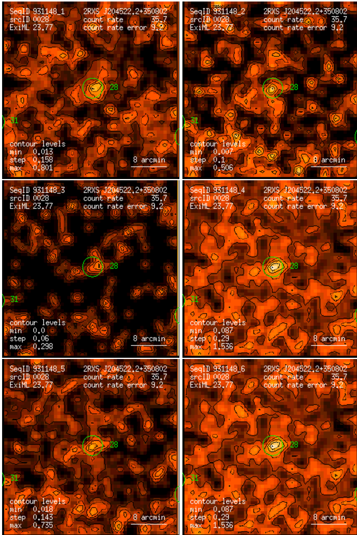
Figure 28: RASS 931148: detection 0028: band rate images, Gaussian filter: (1) PSPC channels 11 – 41, (2) 52 – 90, (3) 91 – 201, (4) 11 – 235, (5) 52 – 201, (6) 11 – 201. Broad band rates in counts/ks. Band rate contour levels in counts/ks/arcmin 2 .
