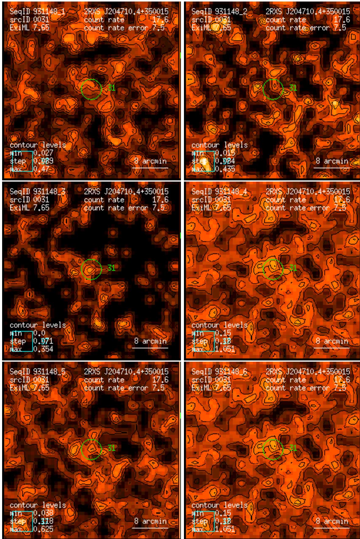
Figure 31: RASS 931148: detection 0031: band rate images, Gaussian filter: (1) PSPC channels 11 – 41, (2) 52 – 90, (3) 91 – 201, (4) 11 – 235, (5) 52 – 201, (6) 11 – 201. Broad band rates in counts/ks. Band rate contour levels in counts/ks/arcmin 2 .
