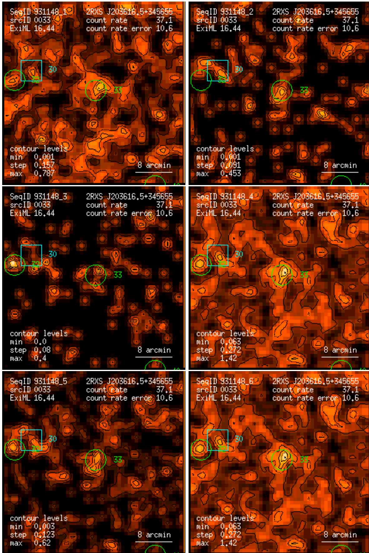
Figure 33: RASS 931148: detection 0033: band rate images, Gaussian filter: (1) PSPC channels 11 – 41, (2) 52 – 90, (3) 91 – 201, (4) 11 – 235, (5) 52 – 201, (6) 11 – 201. Broad band rates in counts/ks. Band rate contour levels in counts/ks/arcmin 2 .
