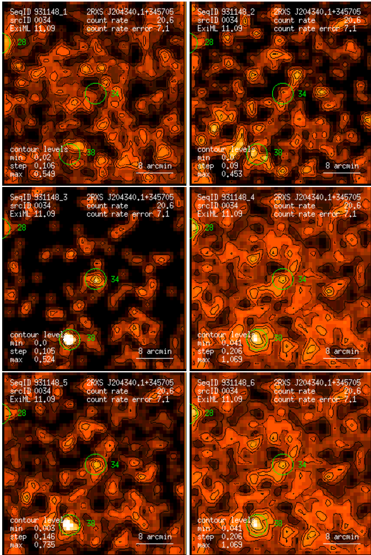
Figure 34: RASS 931148: detection 0034: band rate images, Gaussian filter: (1) PSPC channels 11 – 41, (2) 52 – 90, (3) 91 – 201, (4) 11 – 235, (5) 52 – 201, (6) 11 – 201. Broad band rates in counts/ks. Band rate contour levels in counts/ks/arcmin 2 .
