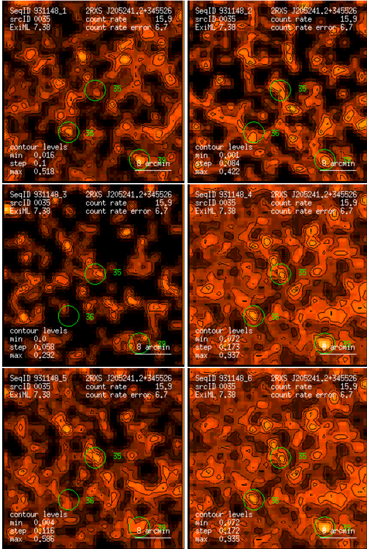
Figure 35: RASS 931148: detection 0035: band rate images, Gaussian filter: (1) PSPC channels 11 – 41, (2) 52 – 90, (3) 91 – 201, (4) 11 – 235, (5) 52 – 201, (6) 11 – 201. Broad band rates in counts/ks. Band rate contour levels in counts/ks/arcmin 2 .
