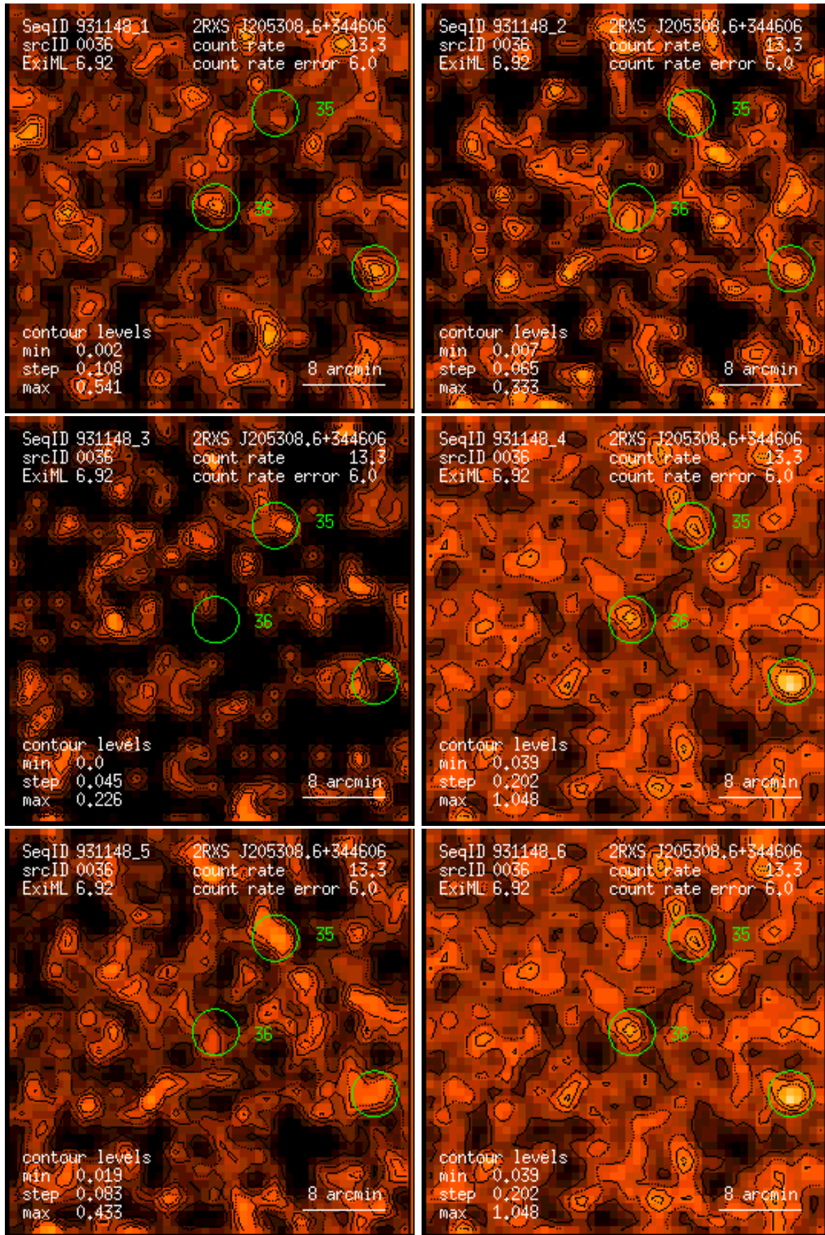
Figure 36: RASS 931148: detection 0036: band rate images, Gaussian filter: (1) PSPC channels 11 – 41, (2) 52 – 90, (3) 91 – 201, (4) 11 – 235, (5) 52 – 201, (6) 11 – 201. Broad band rates in counts/ks. Band rate contour levels in counts/ks/arcmin 2 .
