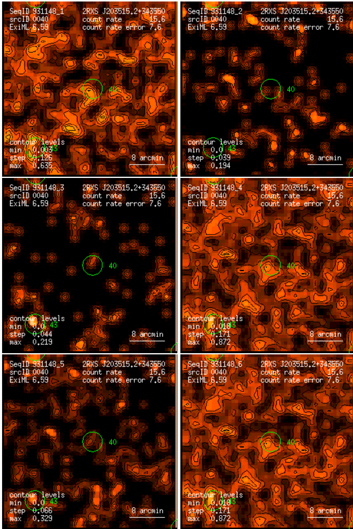
Figure 40: RASS 931148: detection 0040: band rate images, Gaussian filter: (1) PSPC channels 11 – 41, (2) 52 – 90, (3) 91 – 201, (4) 11 – 235, (5) 52 – 201, (6) 11 – 201. Broad band rates in counts/ks. Band rate contour levels in counts/ks/arcmin 2 .
