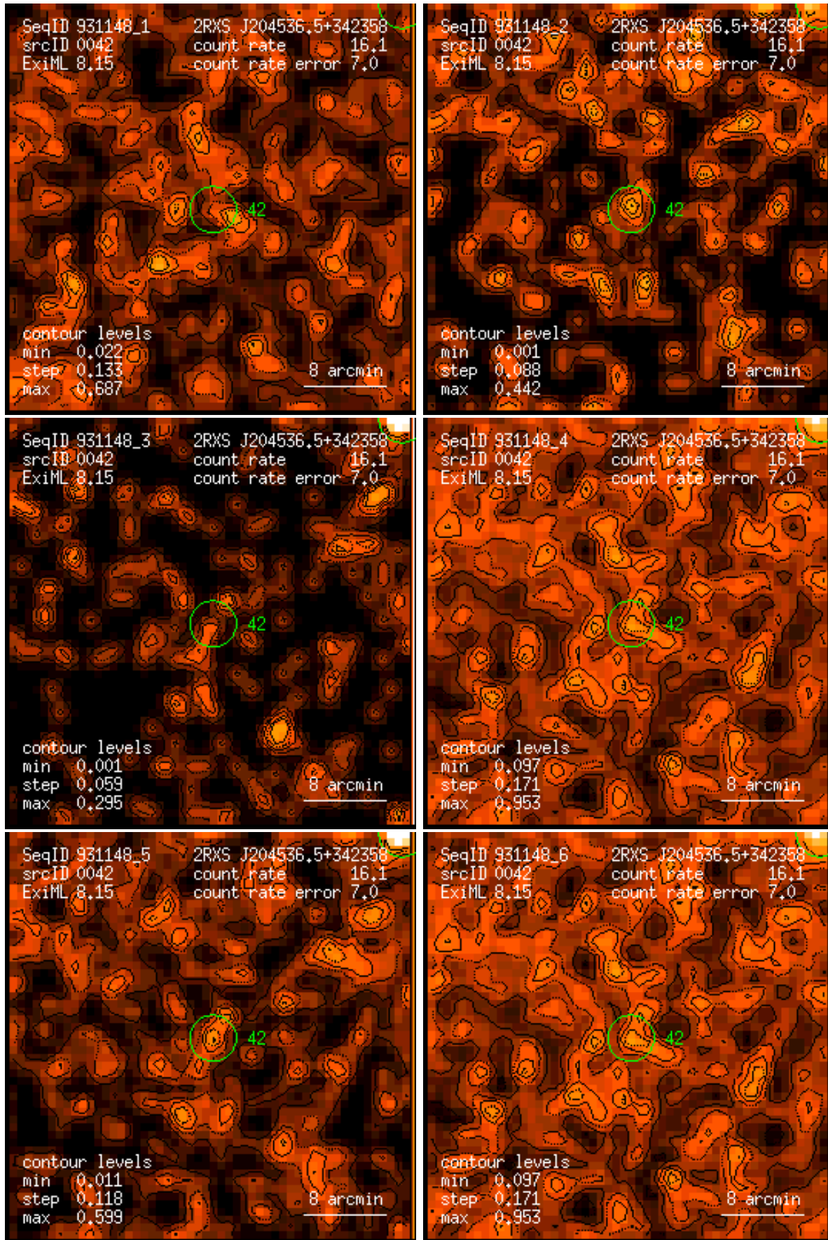
Figure 42: RASS 931148: detection 0042: band rate images, Gaussian filter: (1) PSPC channels 11 – 41, (2) 52 – 90, (3) 91 – 201, (4) 11 – 235, (5) 52 – 201, (6) 11 – 201. Broad band rates in counts/ks. Band rate contour levels in counts/ks/arcmin 2 .
