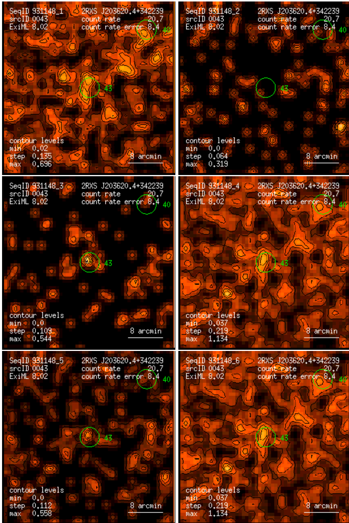
Figure 43: RASS 931148: detection 0043: band rate images, Gaussian filter: (1) PSPC channels 11 – 41, (2) 52 – 90, (3) 91 – 201, (4) 11 – 235, (5) 52 – 201, (6) 11 – 201. Broad band rates in counts/ks. Band rate contour levels in counts/ks/arcmin 2 .
