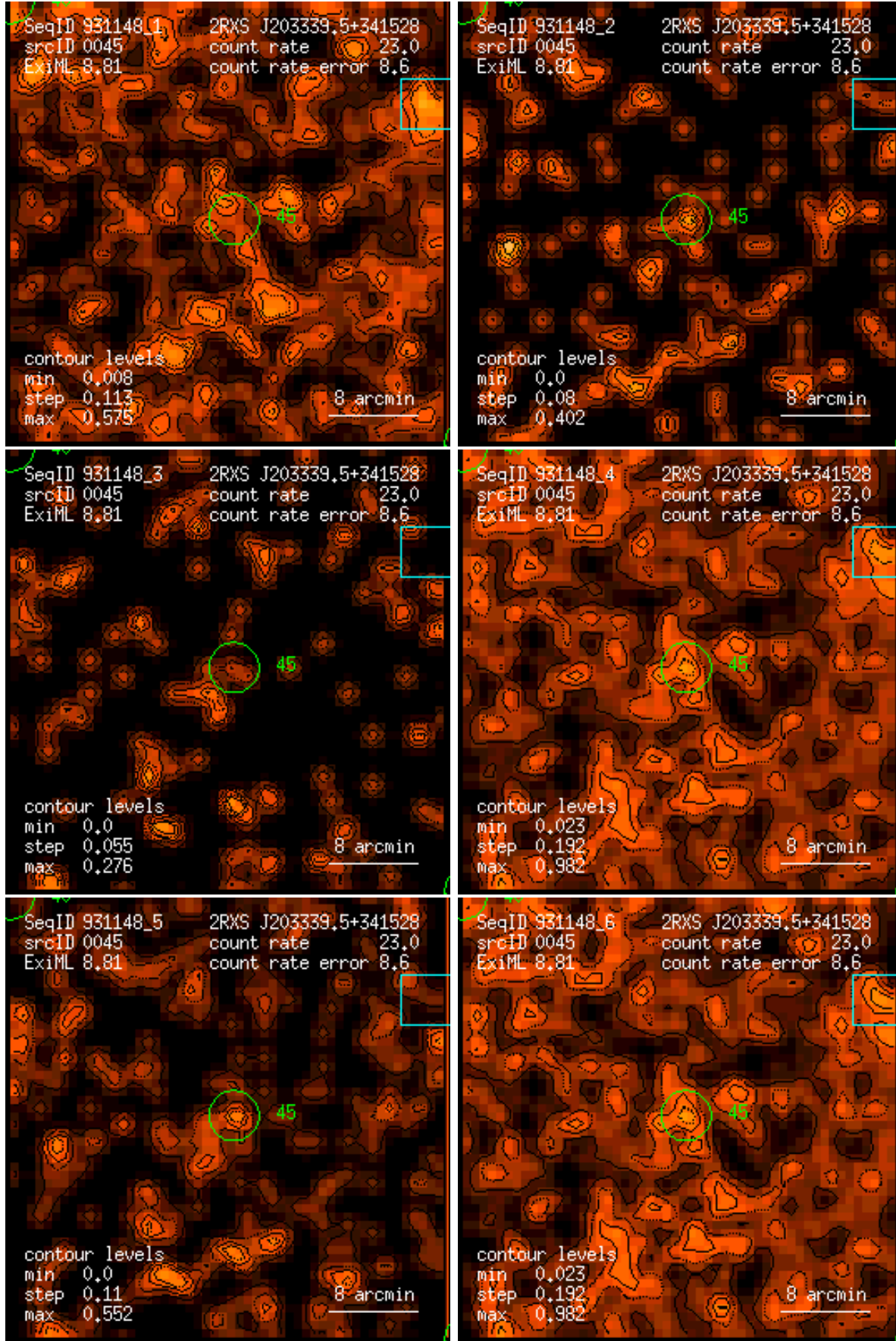
Figure 45: RASS 931148: detection 0045: band rate images, Gaussian filter: (1) PSPC channels 11 – 41, (2) 52 – 90, (3) 91 – 201, (4) 11 – 235, (5) 52 – 201, (6) 11 – 201. Broad band rates in counts/ks. Band rate contour levels in counts/ks/arcmin 2 .
