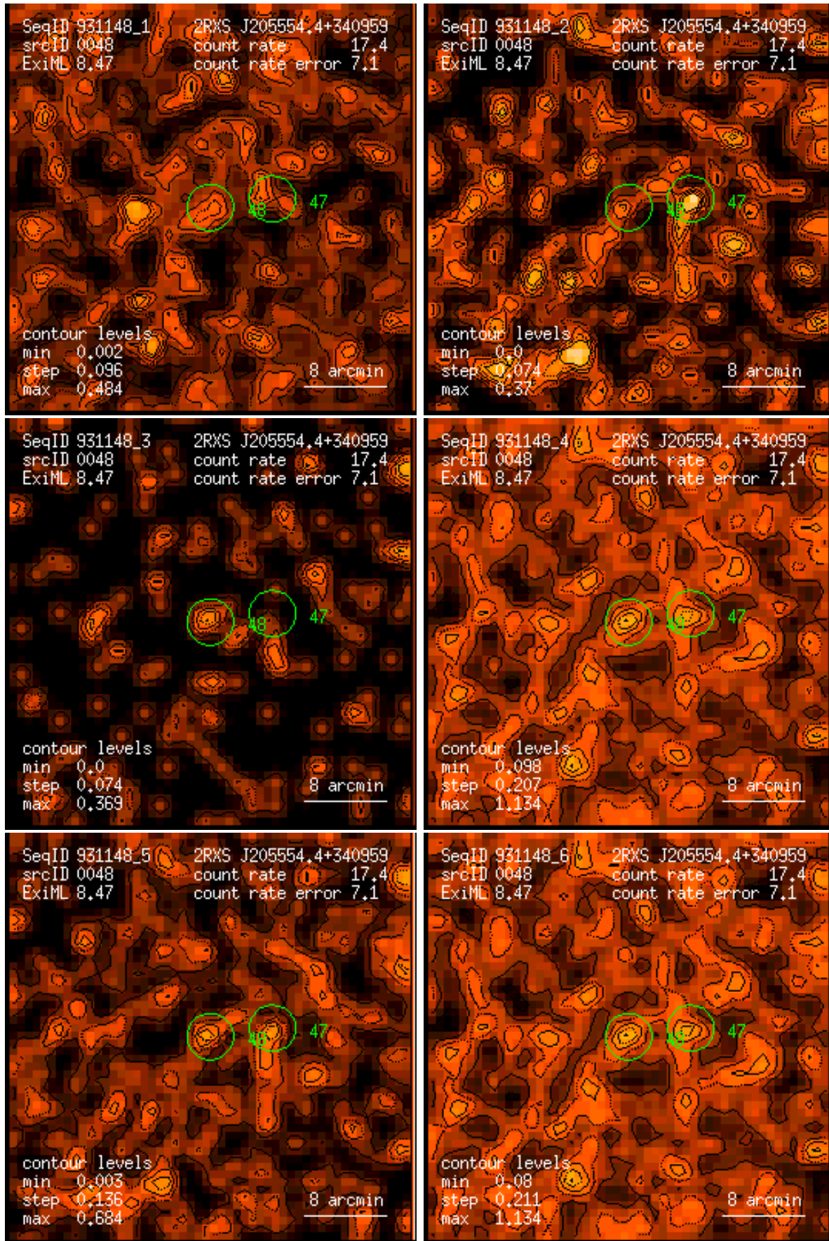
Figure 48: RASS 931148: detection 0048: band rate images, Gaussian filter: (1) PSPC channels 11 – 41, (2) 52 – 90, (3) 91 – 201, (4) 11 – 235, (5) 52 – 201, (6) 11 – 201. Broad band rates in counts/ks. Band rate contour levels in counts/ks/arcmin 2 .
