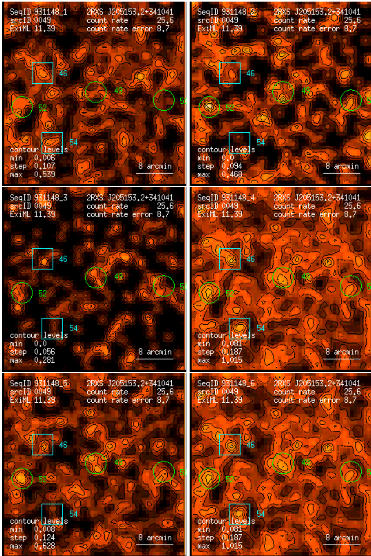
Figure 49: RASS 931148: detection 0049: band rate images, Gaussian filter: (1) PSPC channels 11 – 41, (2) 52 – 90, (3) 91 – 201, (4) 11 – 235, (5) 52 – 201, (6) 11 – 201. Broad band rates in counts/ks. Band rate contour levels in counts/ks/arcmin 2 .
