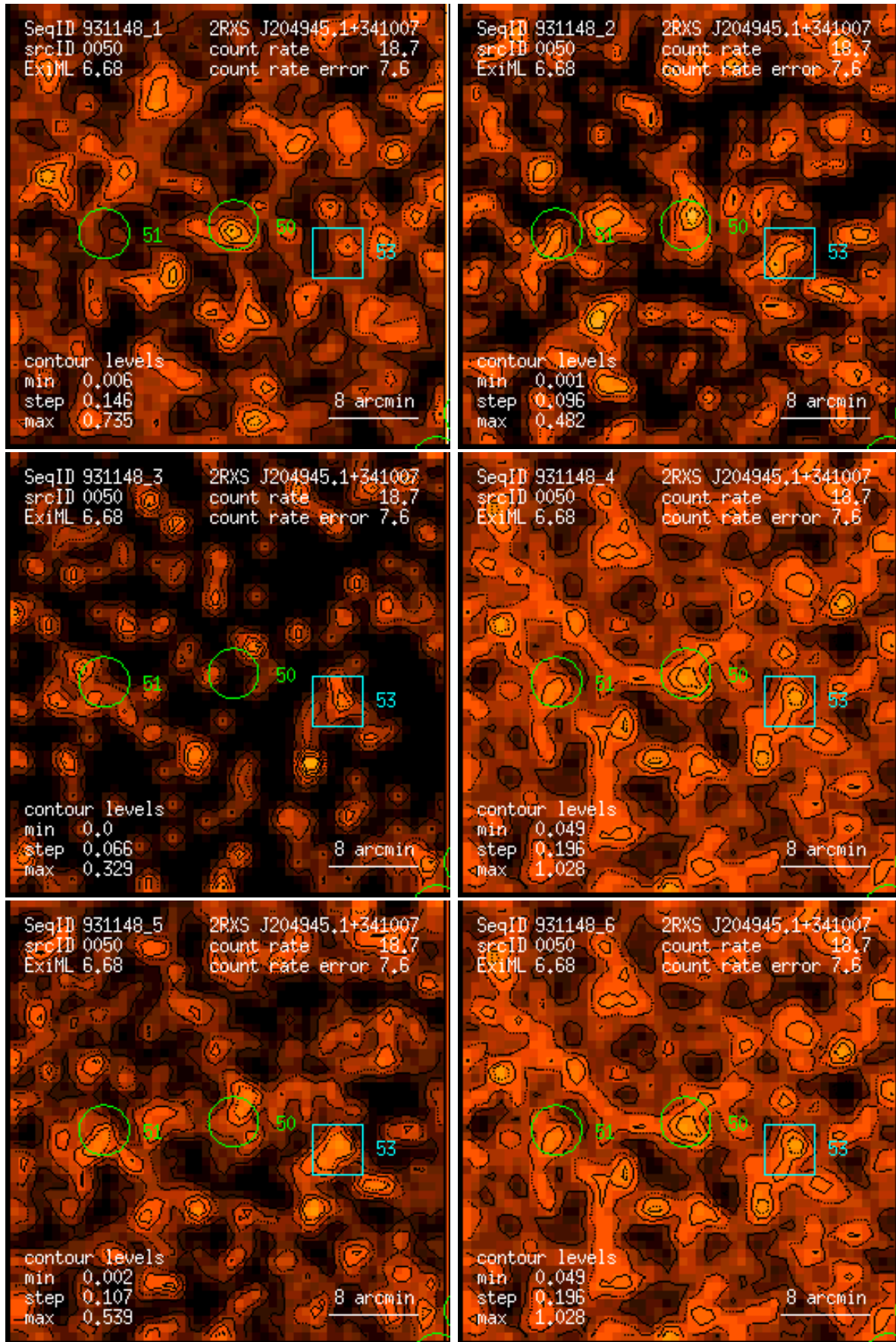
Figure 50: RASS 931148: detection 0050: band rate images, Gaussian filter: (1) PSPC channels 11 – 41, (2) 52 – 90, (3) 91 – 201, (4) 11 – 235, (5) 52 – 201, (6) 11 – 201. Broad band rates in counts/ks. Band rate contour levels in counts/ks/arcmin 2 .
