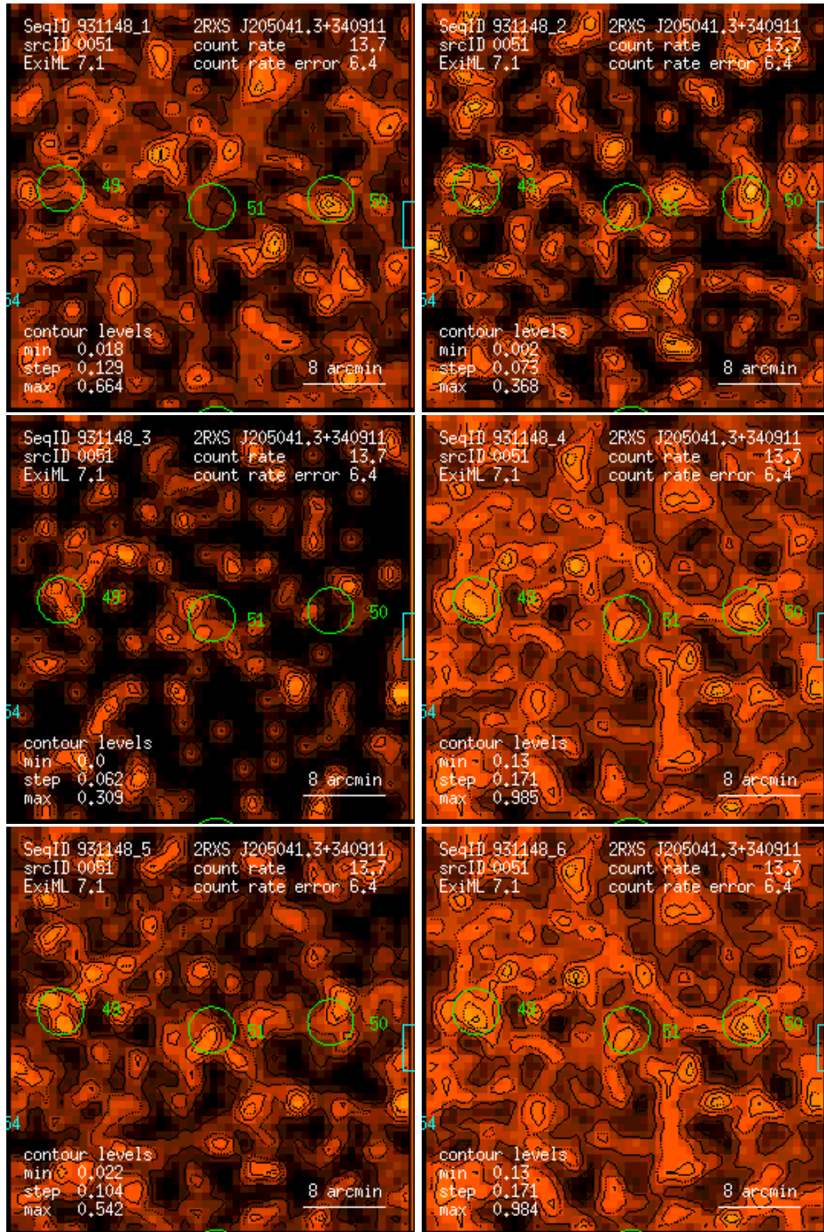
Figure 51: RASS 931148: detection 0051: band rate images, Gaussian filter: (1) PSPC channels 11 – 41, (2) 52 – 90, (3) 91 – 201, (4) 11 – 235, (5) 52 – 201, (6) 11 – 201. Broad band rates in counts/ks. Band rate contour levels in counts/ks/arcmin 2 .
