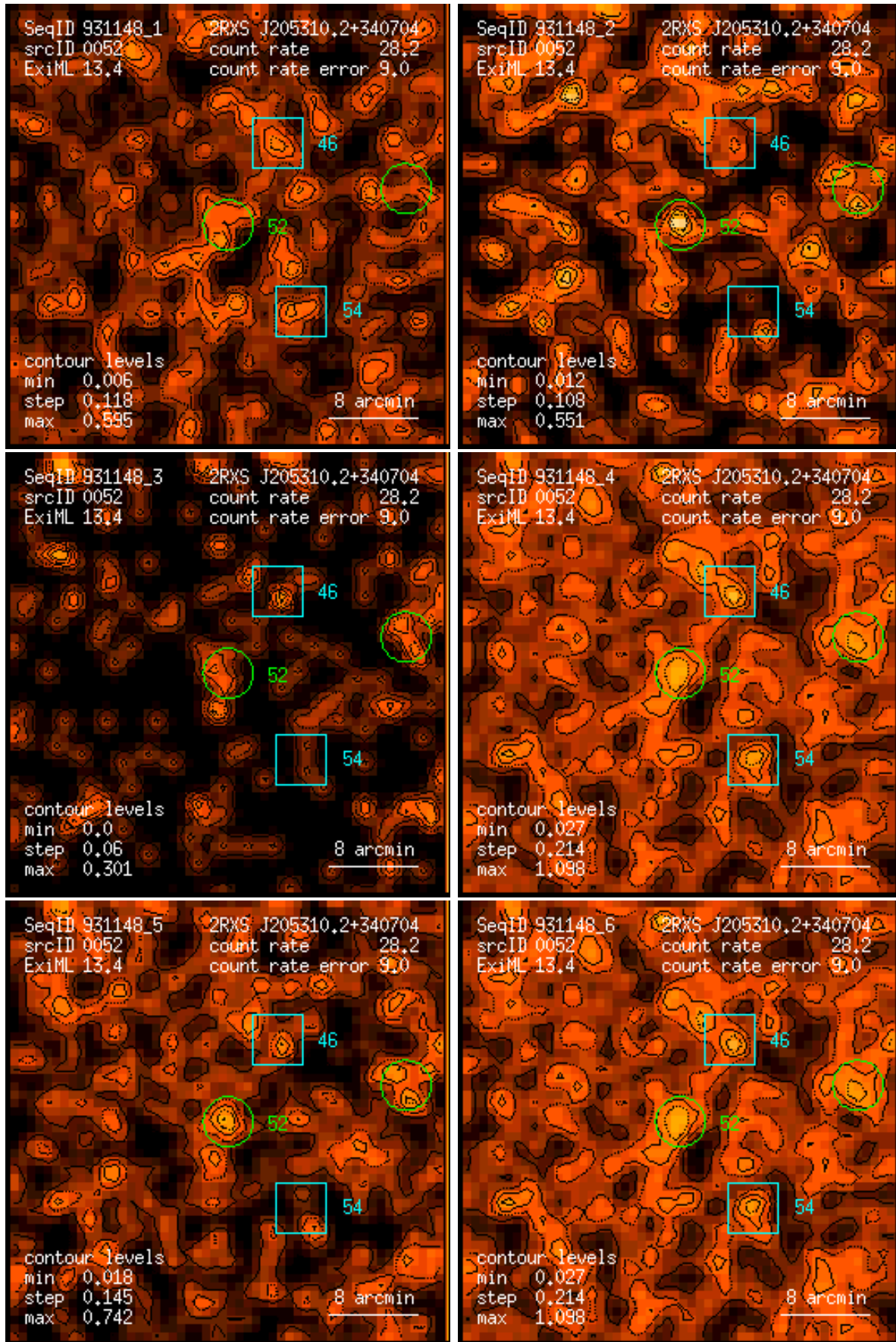
Figure 52: RASS 931148: detection 0052: band rate images, Gaussian filter: (1) PSPC channels 11 – 41, (2) 52 – 90, (3) 91 – 201, (4) 11 – 235, (5) 52 – 201, (6) 11 – 201. Broad band rates in counts/ks. Band rate contour levels in counts/ks/arcmin 2 .
