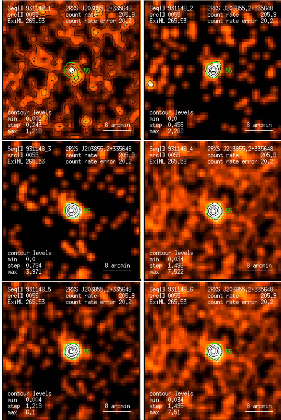
Figure 55: RASS 931148: detection 0055: band rate images, Gaussian filter: (1) PSPC channels 11 – 41, (2) 52 – 90, (3) 91 – 201, (4) 11 – 235, (5) 52 – 201, (6) 11 – 201. Broad band rates in counts/ks. Band rate contour levels in counts/ks/arcmin 2 .
