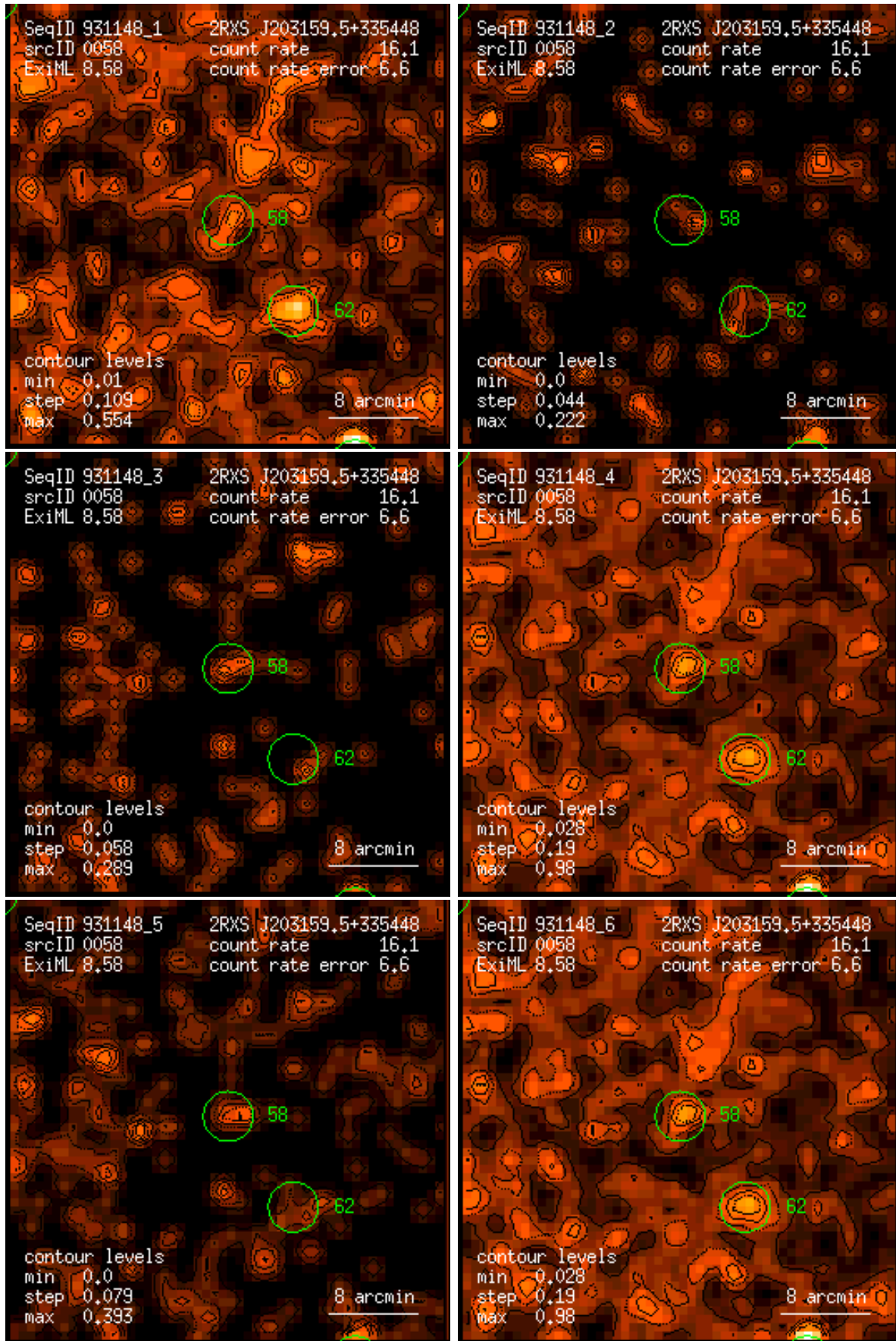
Figure 58: RASS 931148: detection 0058: band rate images, Gaussian filter: (1) PSPC channels 11 – 41, (2) 52 – 90, (3) 91 – 201, (4) 11 – 235, (5) 52 – 201, (6) 11 – 201. Broad band rates in counts/ks. Band rate contour levels in counts/ks/arcmin 2 .
