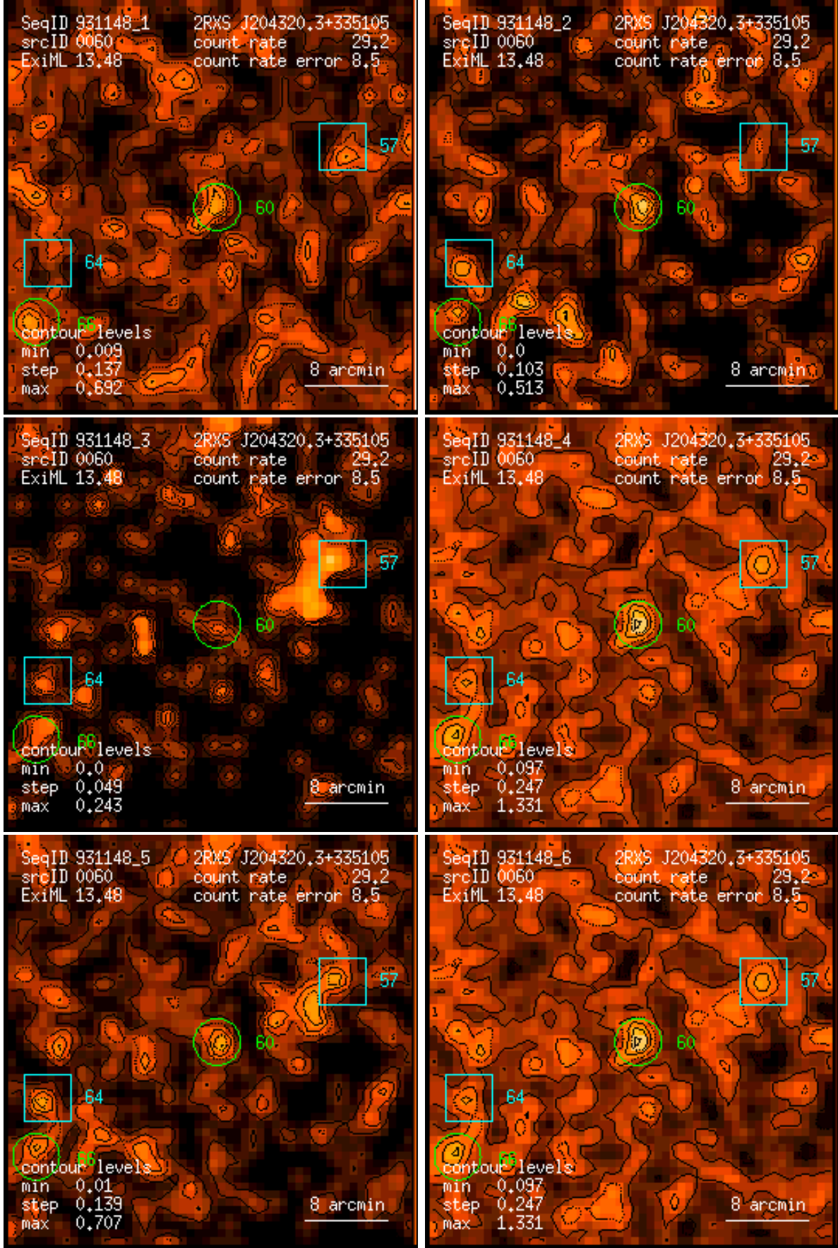
Figure 60: RASS 931148: detection 0060: band rate images, Gaussian filter: (1) PSPC channels 11 – 41, (2) 52 – 90, (3) 91 – 201, (4) 11 – 235, (5) 52 – 201, (6) 11 – 201. Broad band rates in counts/ks. Band rate contour levels in counts/ks/arcmin 2 .
