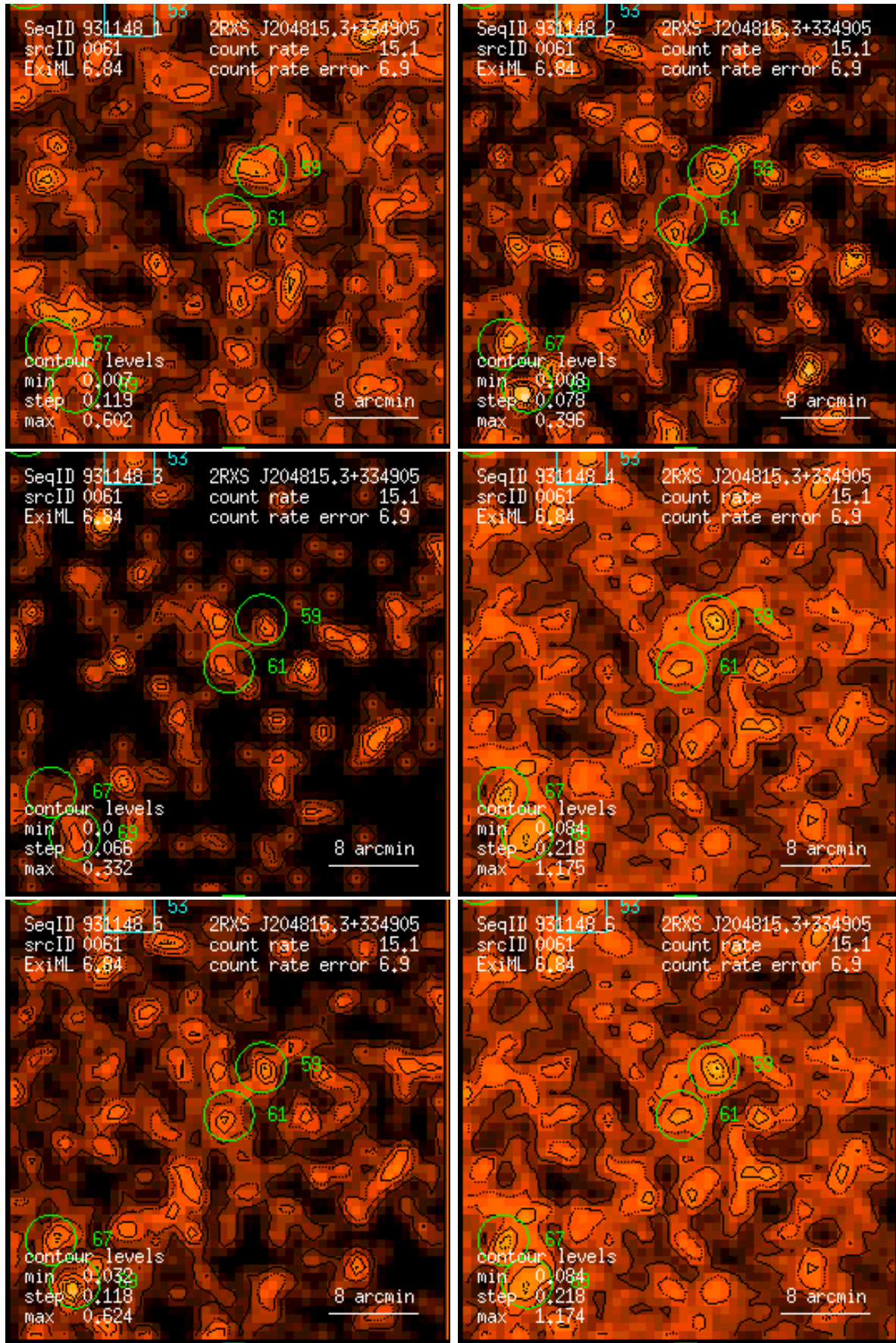
Figure 61: RASS 931148: detection 0061: band rate images, Gaussian filter: (1) PSPC channels 11 – 41, (2) 52 – 90, (3) 91 – 201, (4) 11 – 235, (5) 52 – 201, (6) 11 – 201. Broad band rates in counts/ks. Band rate contour levels in counts/ks/arcmin 2 .
