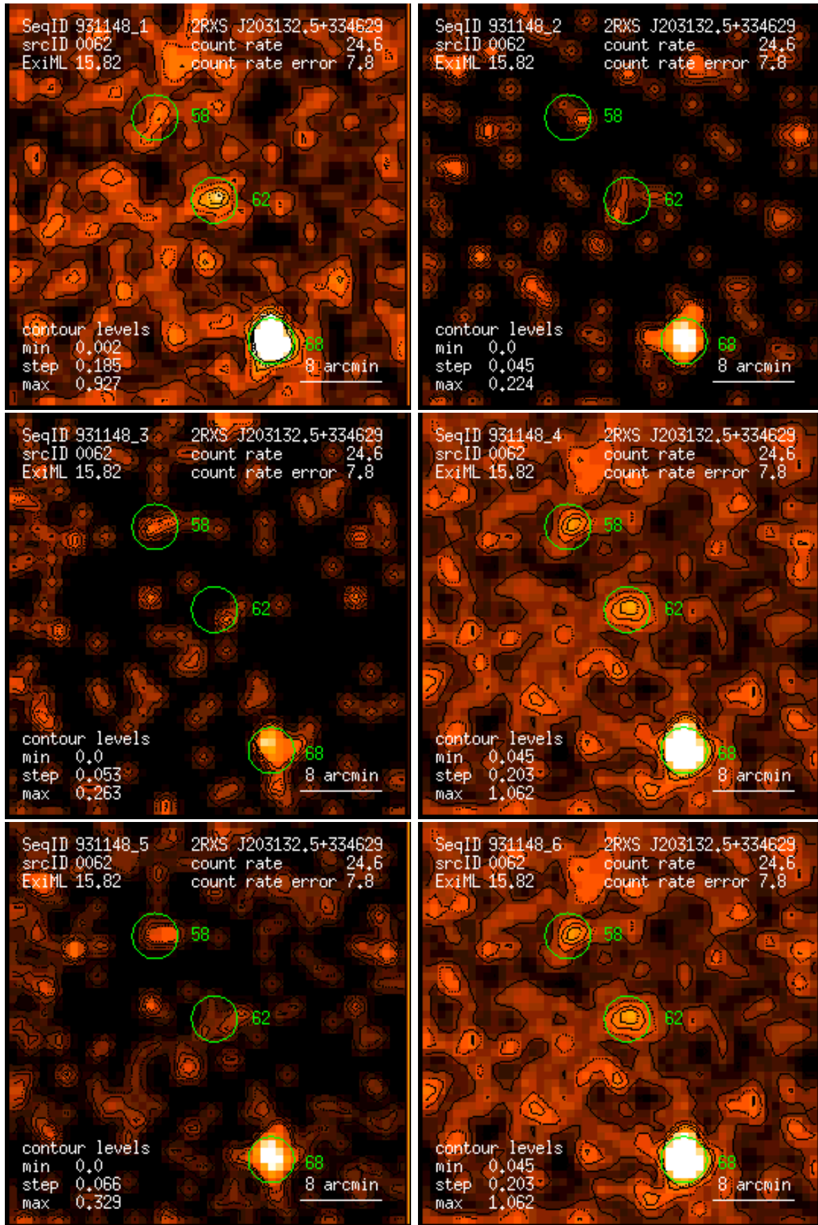
Figure 62: RASS 931148: detection 0062: band rate images, Gaussian filter: (1) PSPC channels 11 – 41, (2) 52 – 90, (3) 91 – 201, (4) 11 – 235, (5) 52 – 201, (6) 11 – 201. Broad band rates in counts/ks. Band rate contour levels in counts/ks/arcmin 2 .
