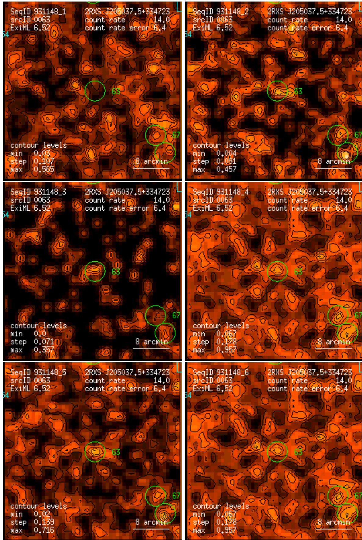
Figure 63: RASS 931148: detection 0063: band rate images, Gaussian filter: (1) PSPC channels 11 – 41, (2) 52 – 90, (3) 91 – 201, (4) 11 – 235, (5) 52 – 201, (6) 11 – 201. Broad band rates in counts/ks. Band rate contour levels in counts/ks/arcmin 2 .
