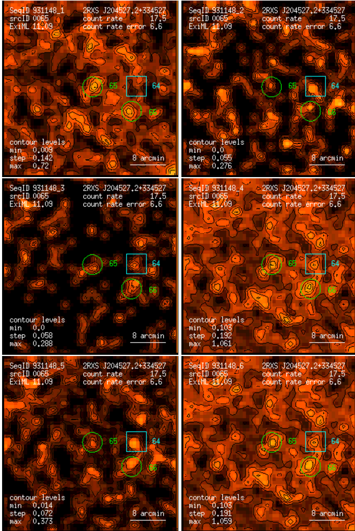
Figure 65: RASS 931148: detection 0065: band rate images, Gaussian filter: (1) PSPC channels 11 – 41, (2) 52 – 90, (3) 91 – 201, (4) 11 – 235, (5) 52 – 201, (6) 11 – 201. Broad band rates in counts/ks. Band rate contour levels in counts/ks/arcmin 2 .
