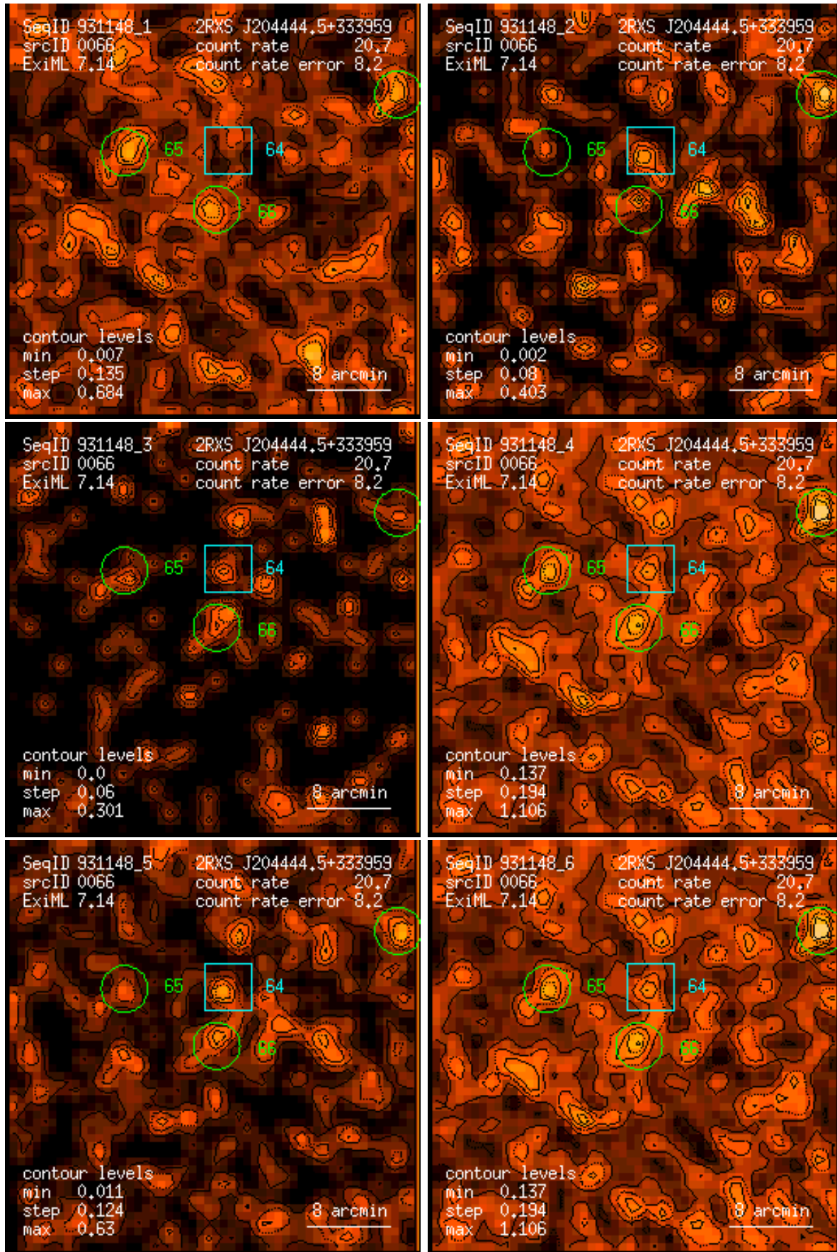
Figure 66: RASS 931148: detection 0066: band rate images, Gaussian filter: (1) PSPC channels 11 – 41, (2) 52 – 90, (3) 91 – 201, (4) 11 – 235, (5) 52 – 201, (6) 11 – 201. Broad band rates in counts/ks. Band rate contour levels in counts/ks/arcmin 2 .
