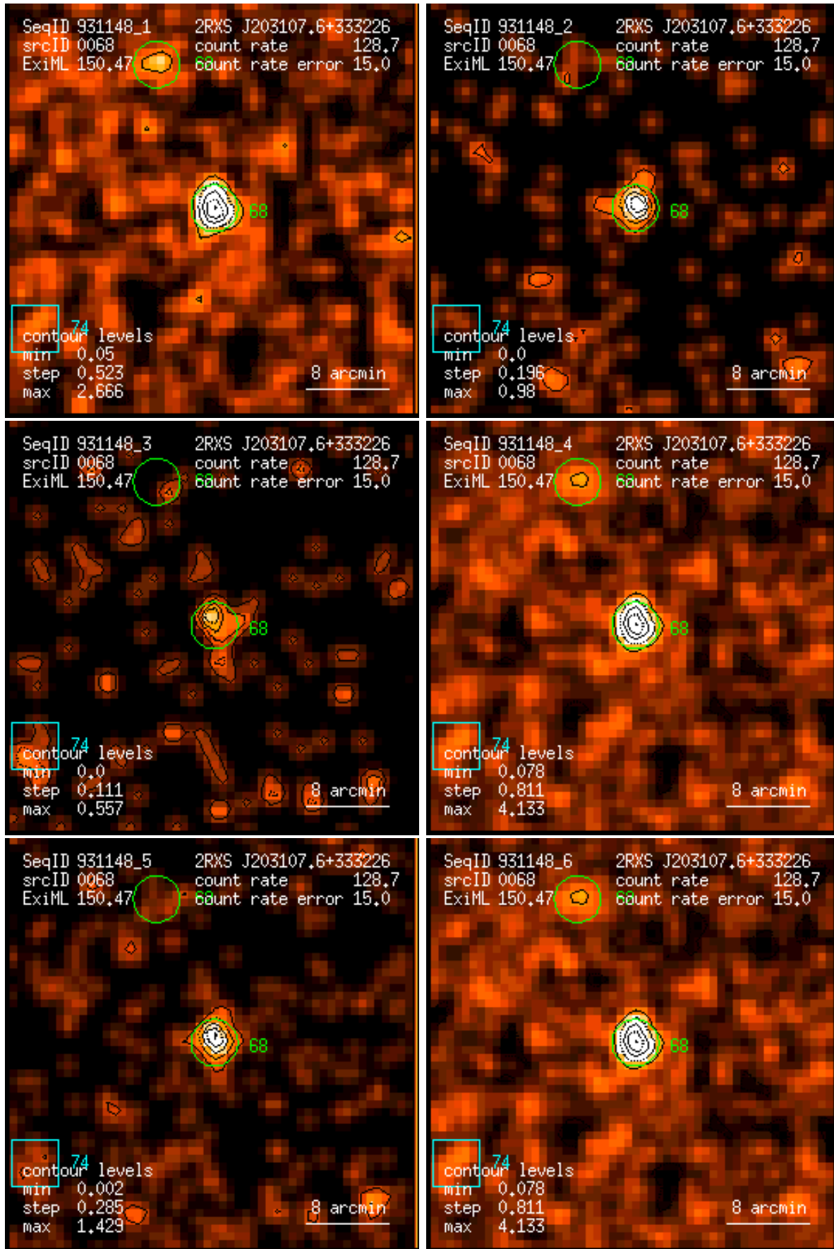
Figure 68: RASS 931148: detection 0068: band rate images, Gaussian filter: (1) PSPC channels 11 – 41, (2) 52 – 90, (3) 91 – 201, (4) 11 – 235, (5) 52 – 201, (6) 11 – 201. Broad band rates in counts/ks. Band rate contour levels in counts/ks/arcmin 2 .
