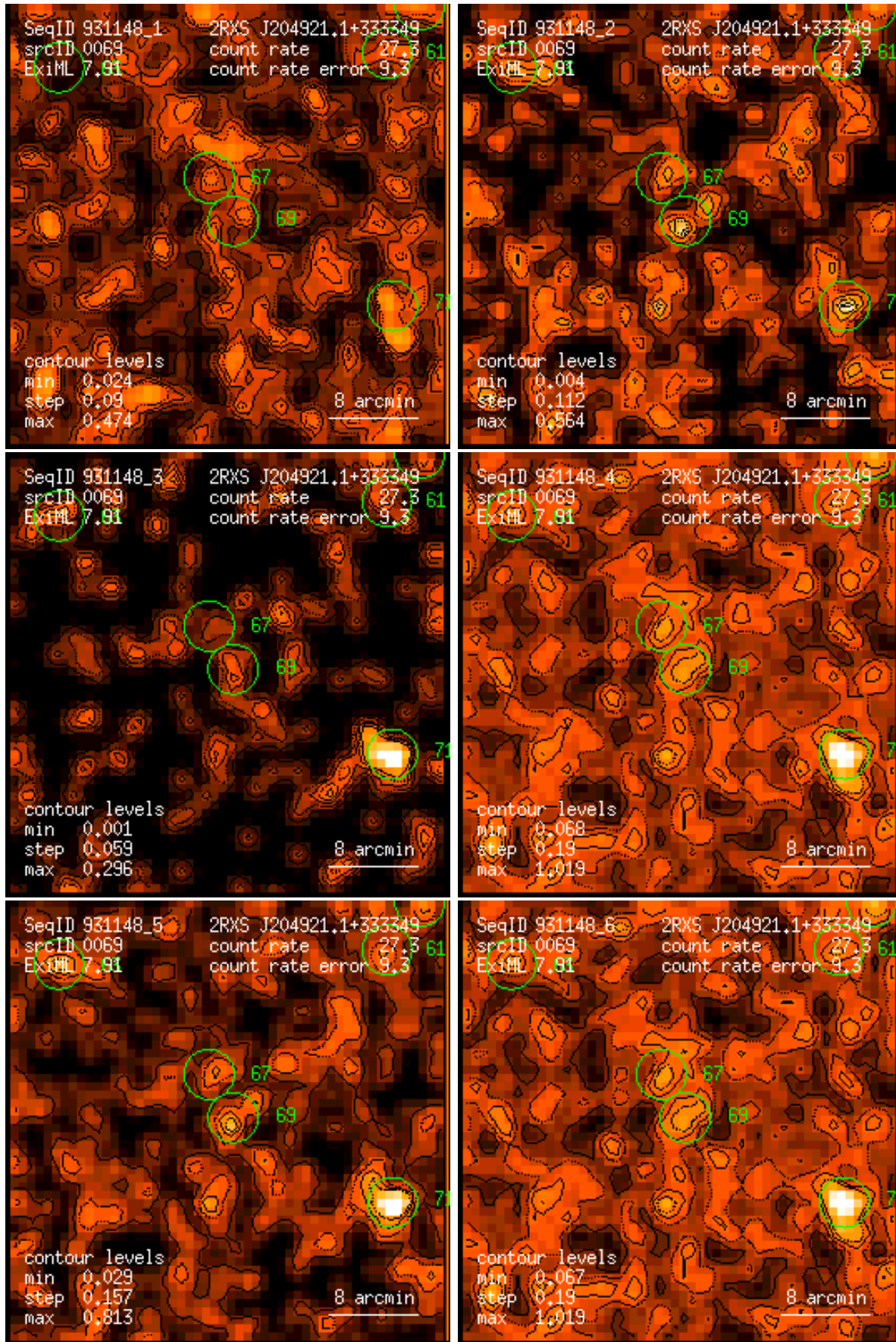
Figure 69: RASS 931148: detection 0069: band rate images, Gaussian filter: (1) PSPC channels 11 – 41, (2) 52 – 90, (3) 91 – 201, (4) 11 – 235, (5) 52 – 201, (6) 11 – 201. Broad band rates in counts/ks. Band rate contour levels in counts/ks/arcmin 2 .
