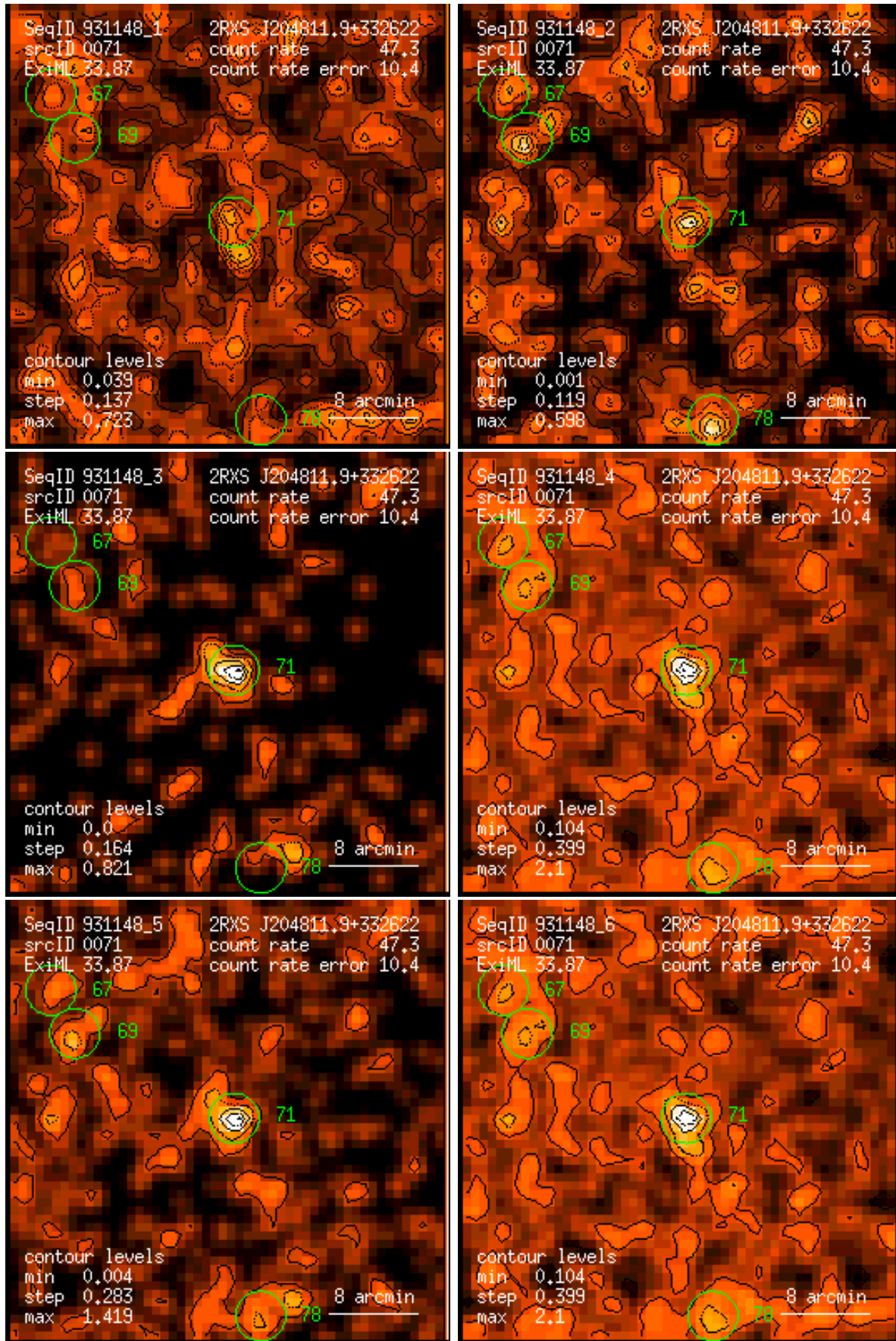
Figure 71: RASS 931148: detection 0071: band rate images, Gaussian filter: (1) PSPC channels 11 – 41, (2) 52 – 90, (3) 91 – 201, (4) 11 – 235, (5) 52 – 201, (6) 11 – 201. Broad band rates in counts/ks. Band rate contour levels in counts/ks/arcmin 2 .
