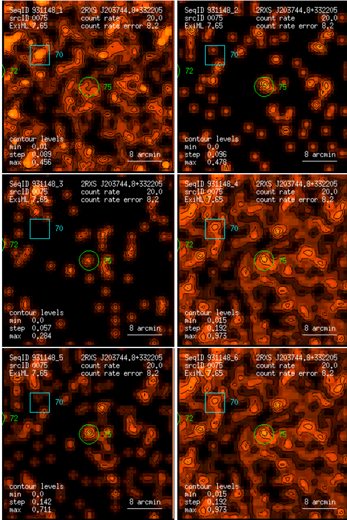
Figure 75: RASS 931148: detection 0075: band rate images, Gaussian filter: (1) PSPC channels 11 – 41, (2) 52 – 90, (3) 91 – 201, (4) 11 – 235, (5) 52 – 201, (6) 11 – 201. Broad band rates in counts/ks. Band rate contour levels in counts/ks/arcmin 2 .
