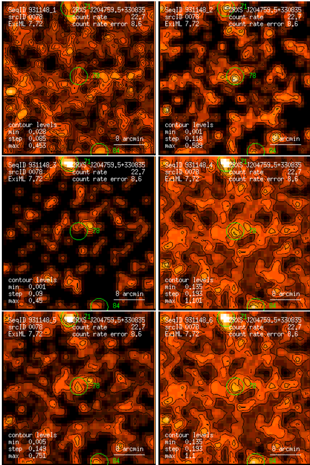
Figure 78: RASS 931148: detection 0078: band rate images, Gaussian filter: (1) PSPC channels 11 – 41, (2) 52 – 90, (3) 91 – 201, (4) 11 – 235, (5) 52 – 201, (6) 11 – 201. Broad band rates in counts/ks. Band rate contour levels in counts/ks/arcmin 2 .
