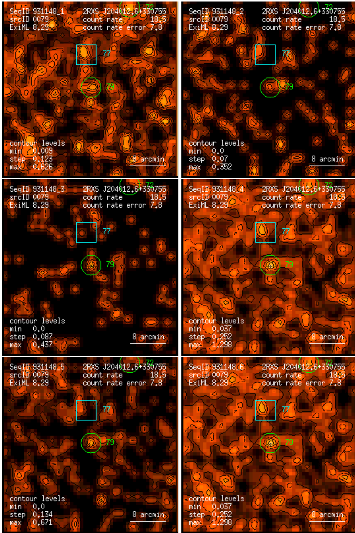
Figure 79: RASS 931148: detection 0079: band rate images, Gaussian filter: (1) PSPC channels 11 – 41, (2) 52 – 90, (3) 91 – 201, (4) 11 – 235, (5) 52 – 201, (6) 11 – 201. Broad band rates in counts/ks. Band rate contour levels in counts/ks/arcmin 2 .
