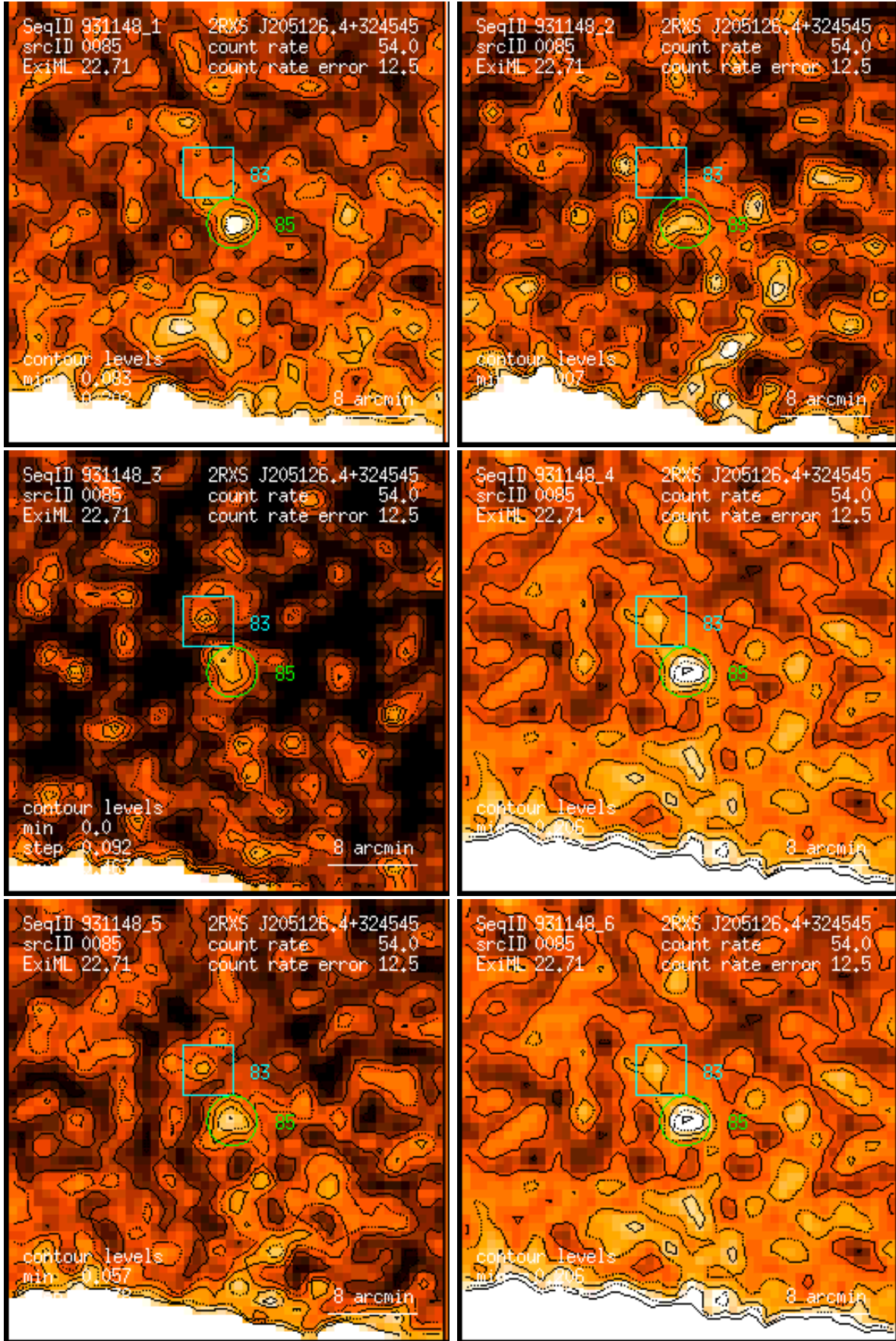
Figure 85: RASS 931148: detection 0085: band rate images, Gaussian filter: (1) PSPC channels 11 – 41, (2) 52 – 90, (3) 91 – 201, (4) 11 – 235, (5) 52 – 201, (6) 11 – 201. Broad band rates in counts/ks. Band rate contour levels in counts/ks/arcmin 2 .
