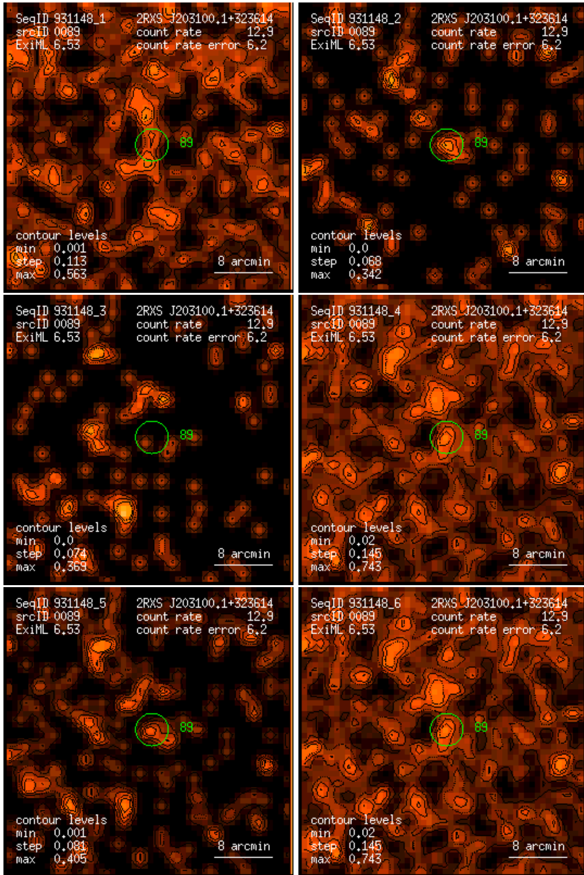
Figure 89: RASS 931148: detection 0089: band rate images, Gaussian filter: (1) PSPC channels 11 – 41, (2) 52 – 90, (3) 91 – 201, (4) 11 – 235, (5) 52 – 201, (6) 11 – 201. Broad band rates in counts/ks. Band rate contour levels in counts/ks/arcmin 2 .
