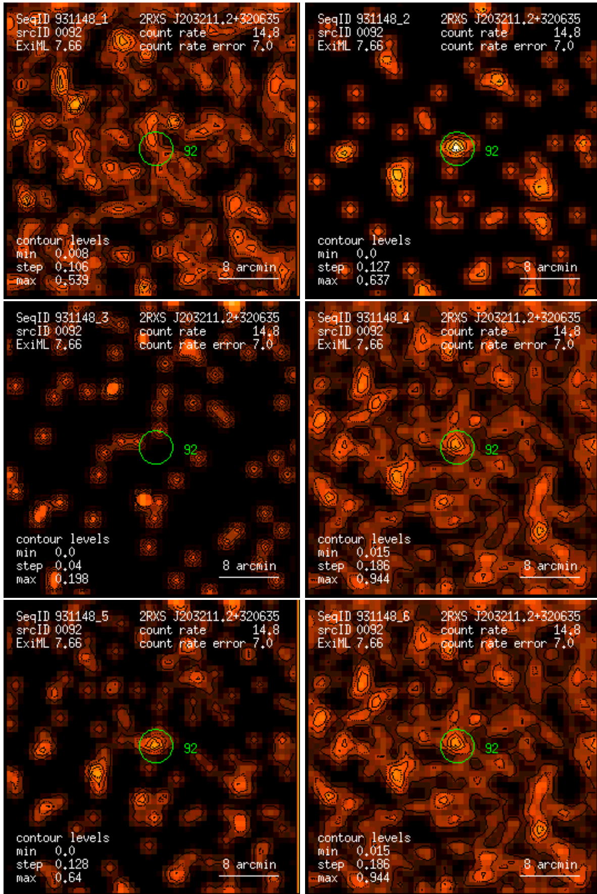
Figure 92: RASS 931148: detection 0092: band rate images, Gaussian filter: (1) PSPC channels 11 – 41, (2) 52 – 90, (3) 91 – 201, (4) 11 – 235, (5) 52 – 201, (6) 11 – 201. Broad band rates in counts/ks. Band rate contour levels in counts/ks/arcmin 2 .
